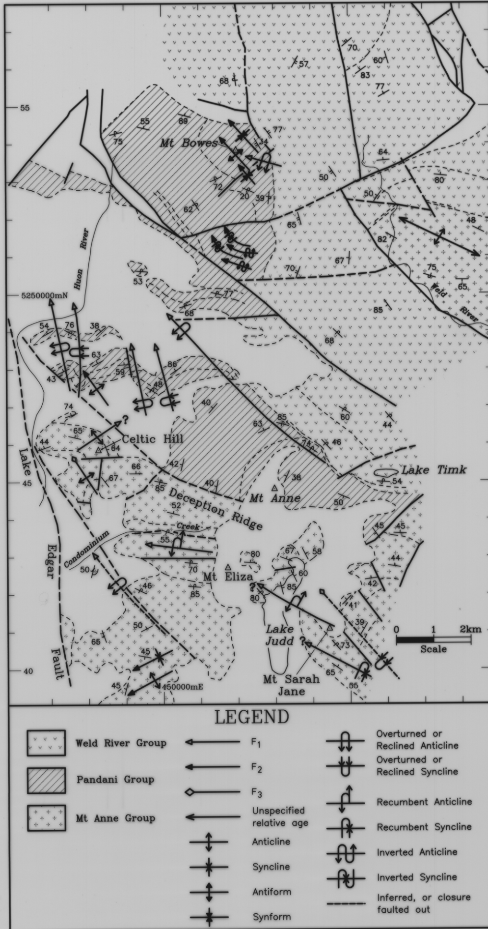
Figure C27. Major folds, Jubilee region. No correlation necessarily implied between Groups.
