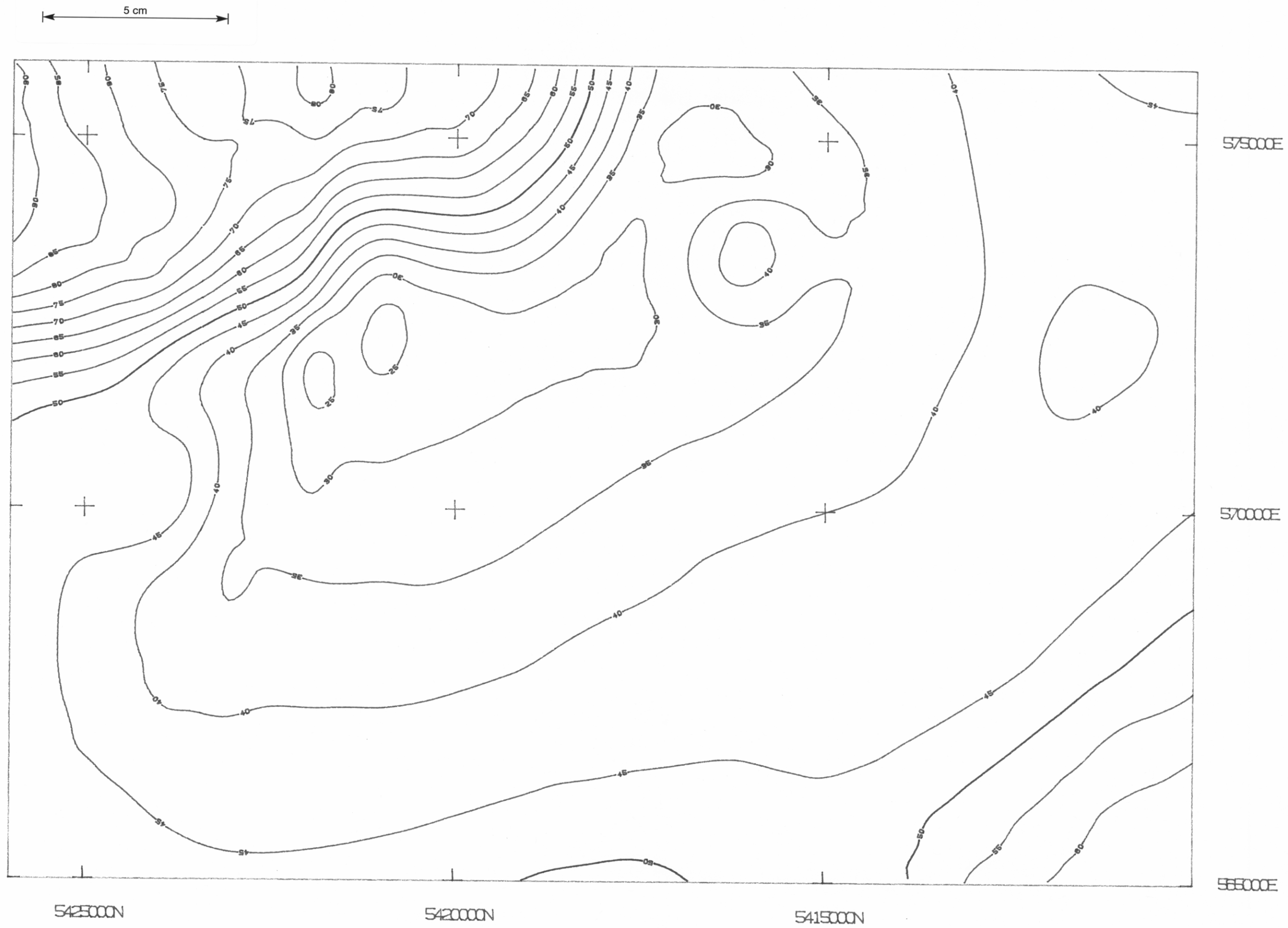
R 1989/37 Fig 4 Magnetic data-1200m terrain clearance (No filter)
