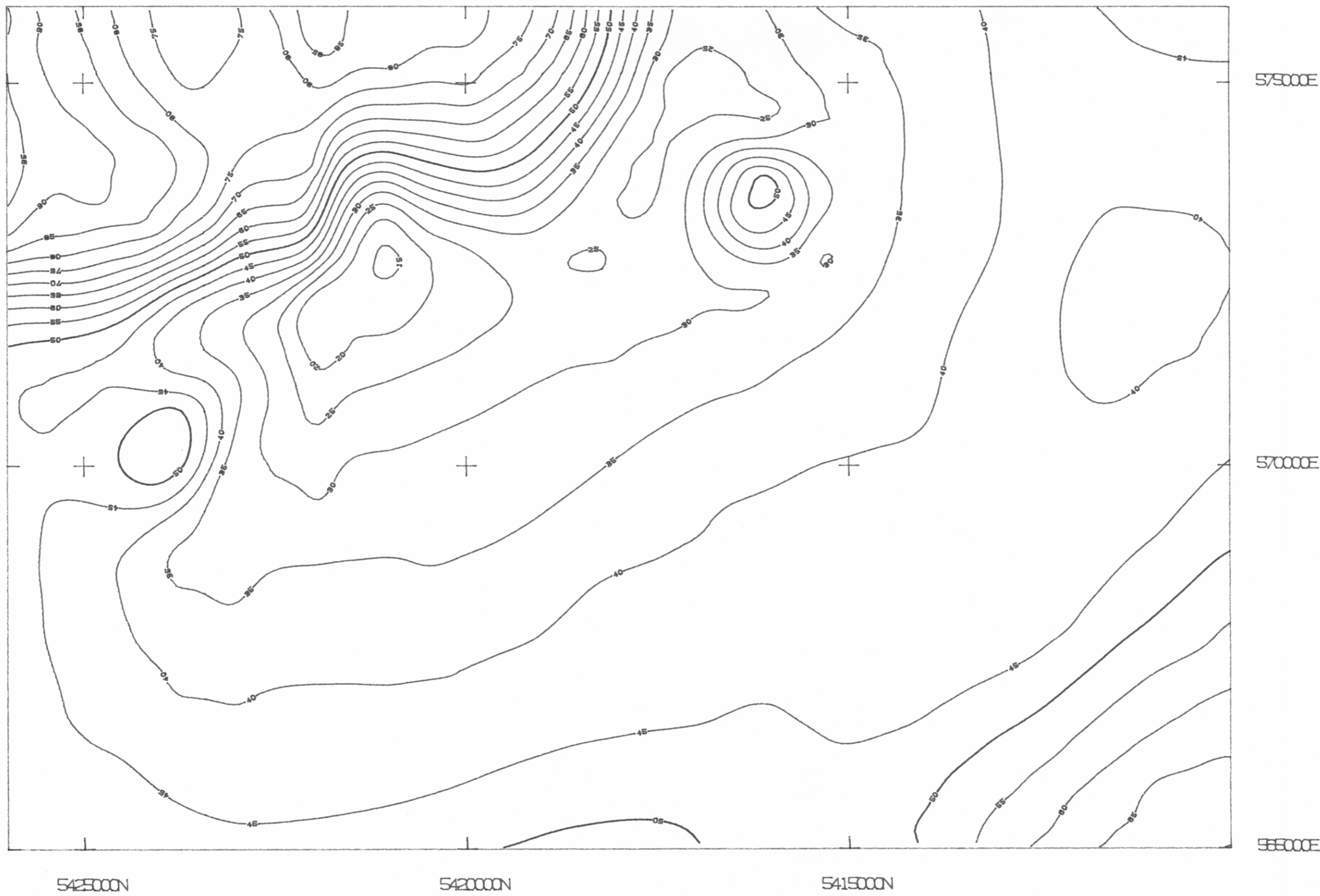
R 1989/37 Fig 5 Magnetic data-900m terrain clearance (No filter)
