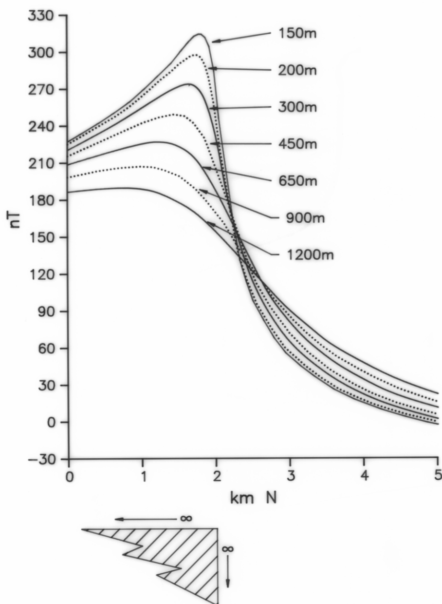
FIG 14 Theoretical anomaly over a fault
