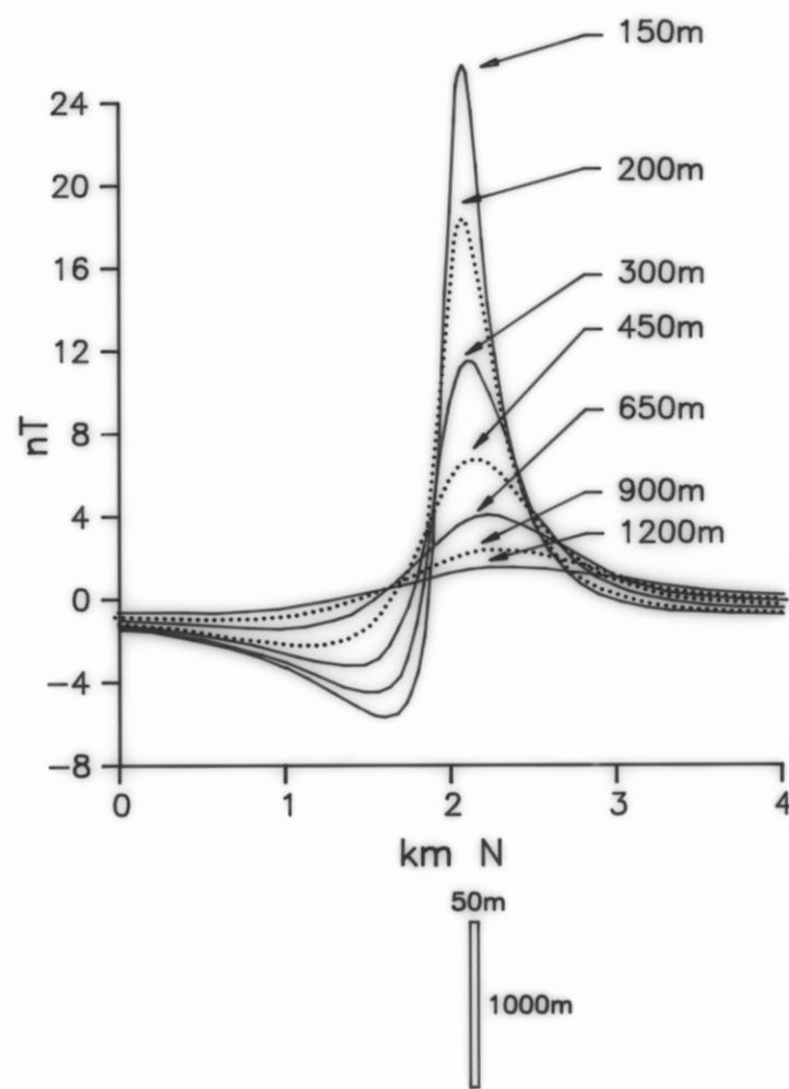
FIG 12 Theoretical anomaly over a thin orebody, 1000m
