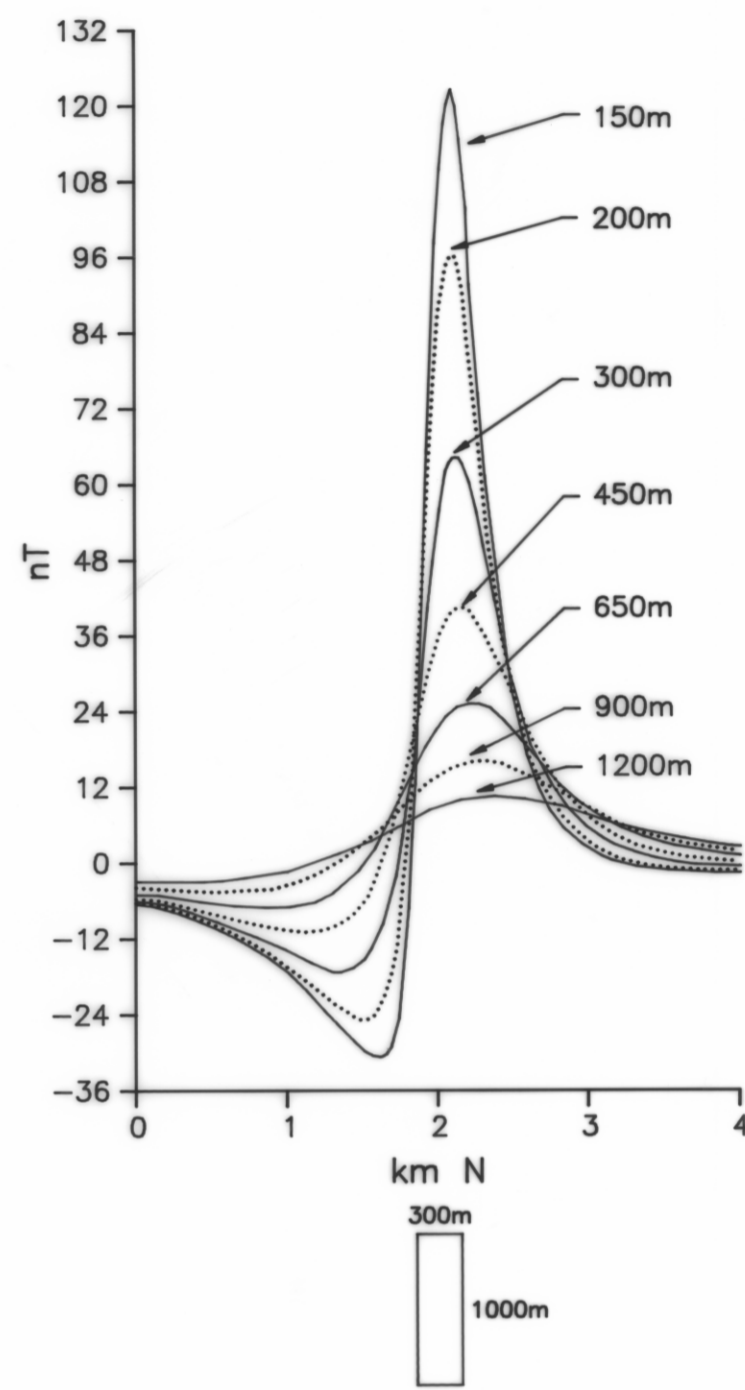
FIG 13 Theoretical anomaly over a thin orebody, 1000m
