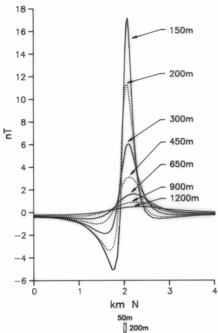
FIG 11 Theoretical anomaly over a thin ore body, 200m
