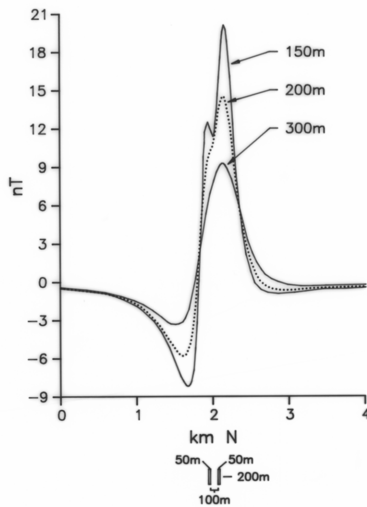
FIG 15 Theoretical anomaly over two thin orebodies, separated horizontally by 200m
