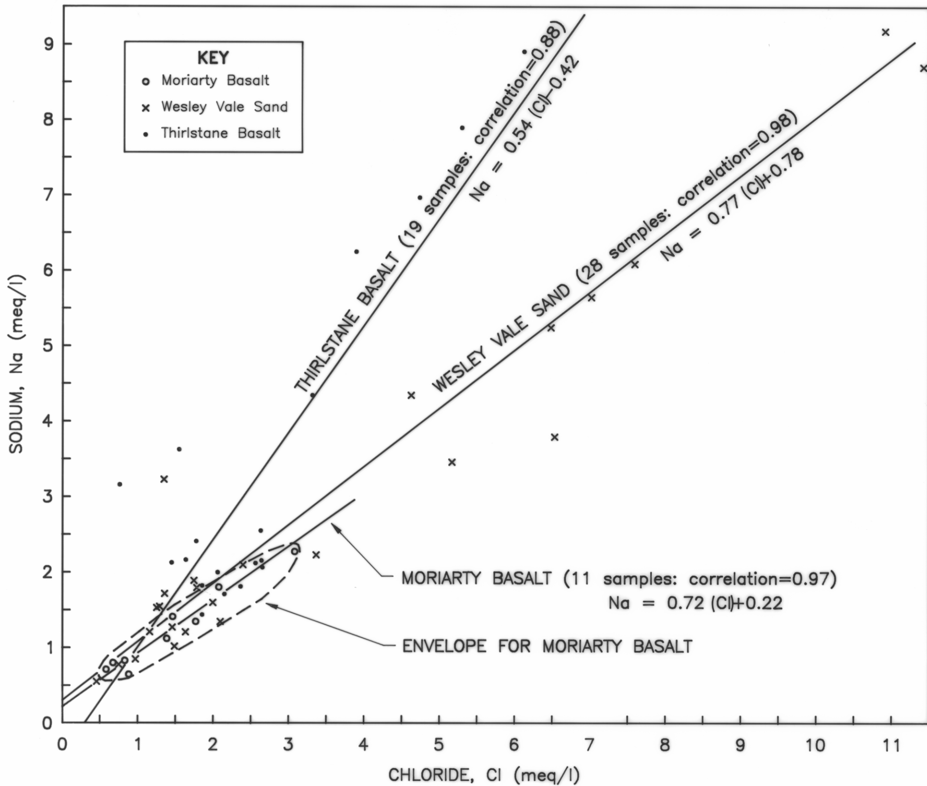
DEVONPORT AREA - SODIUM CHLORIDE VARIATION DIAGRAM FOR GROUNDWATER FROM THE THIRLSTANE & MORIARTY BASALTS AND THE WESLEY VALE SAND FIGURE 25 10 BULL.67 - DEVONPORT GROUNDWATER AUTHOR: W.C. CROMER TASMANIA DEPARTMENT OF MINES, DRAFTSPERSON: J. LADANIWSKYJ 5326 J
