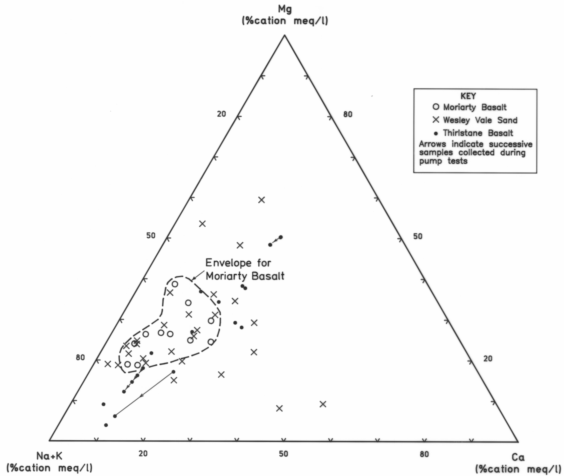
FIG 22 Cation triangular variation diagram for groundwater from the Thirlstane & Moriarty Basalts and Wesley Vale Sand
