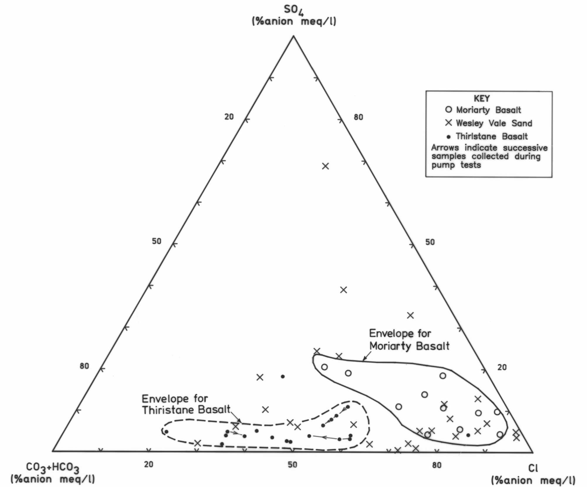
FIG 23 Anion triangular variation diagram for groundwater from the Thirlstane & Moriarty Basalts and Wesley Vale Sand
