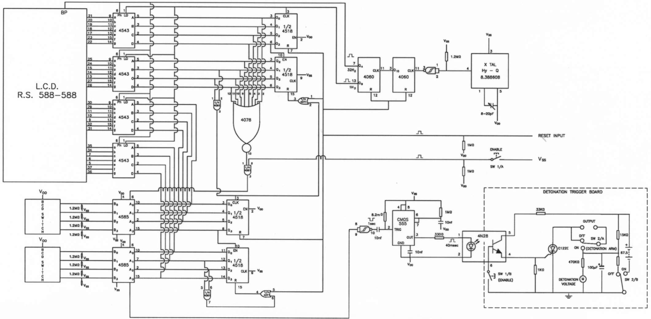
EXPLOSIVE FIRING SHOT BOX CIRCUIT DIAGRAM FIGURE No. REPORT 1990/02 AUTHOR: R.J. SEDGMAN DIVISION OF MINES & MINERAL RESOURCES DRAFTSPERSON: ASM 19/03/90 5332A
