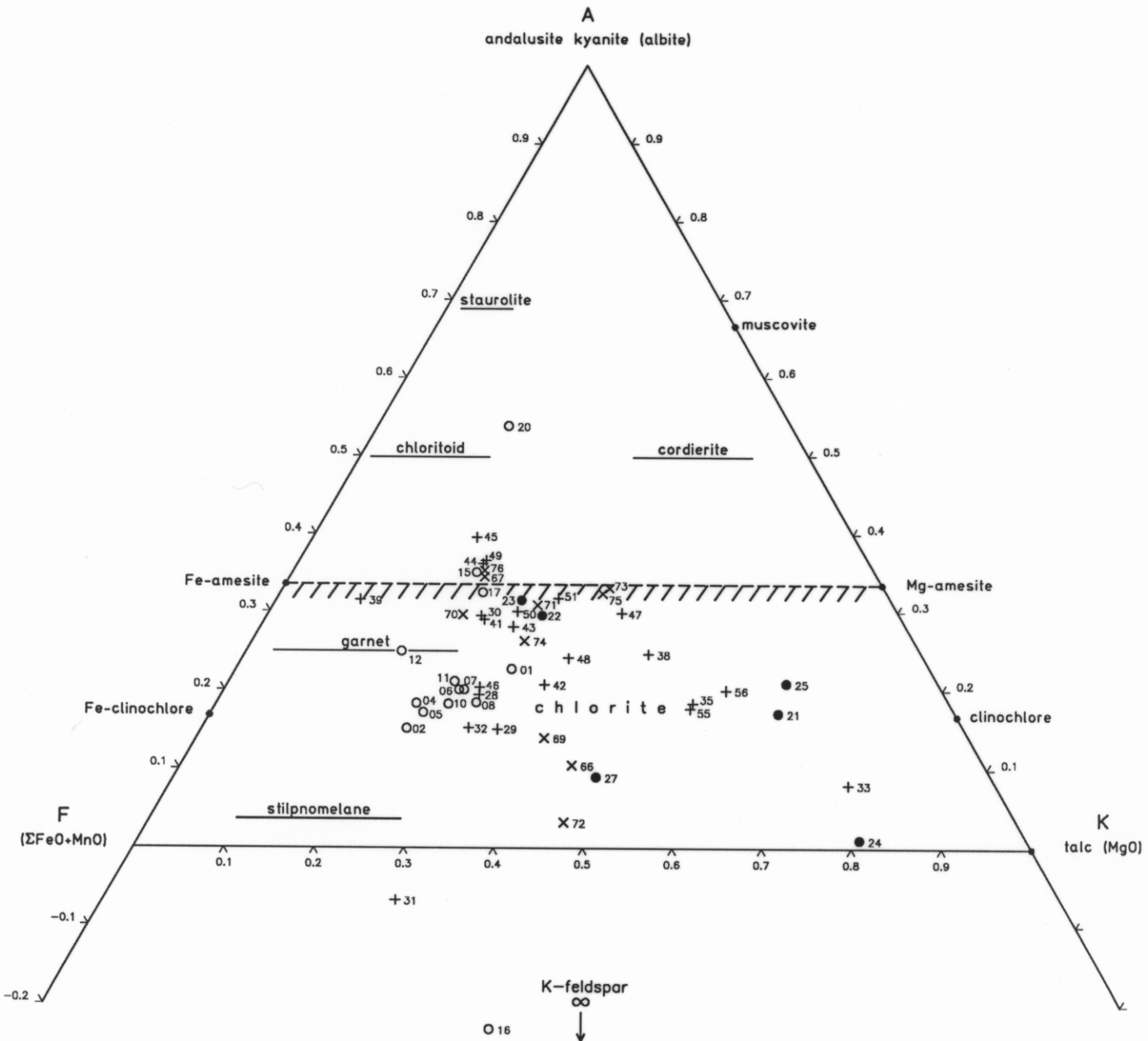
TYENNAN GEANTICLINE, METAPELITES ON AFM DIAGRAM FIGURE No. U/R 1987/07 AUTHOR: J.L. EVERARD DIVISION OF MINES & MINERAL RESOURCES DRAFTSPERSON: ASM 26/02/90 5335C
