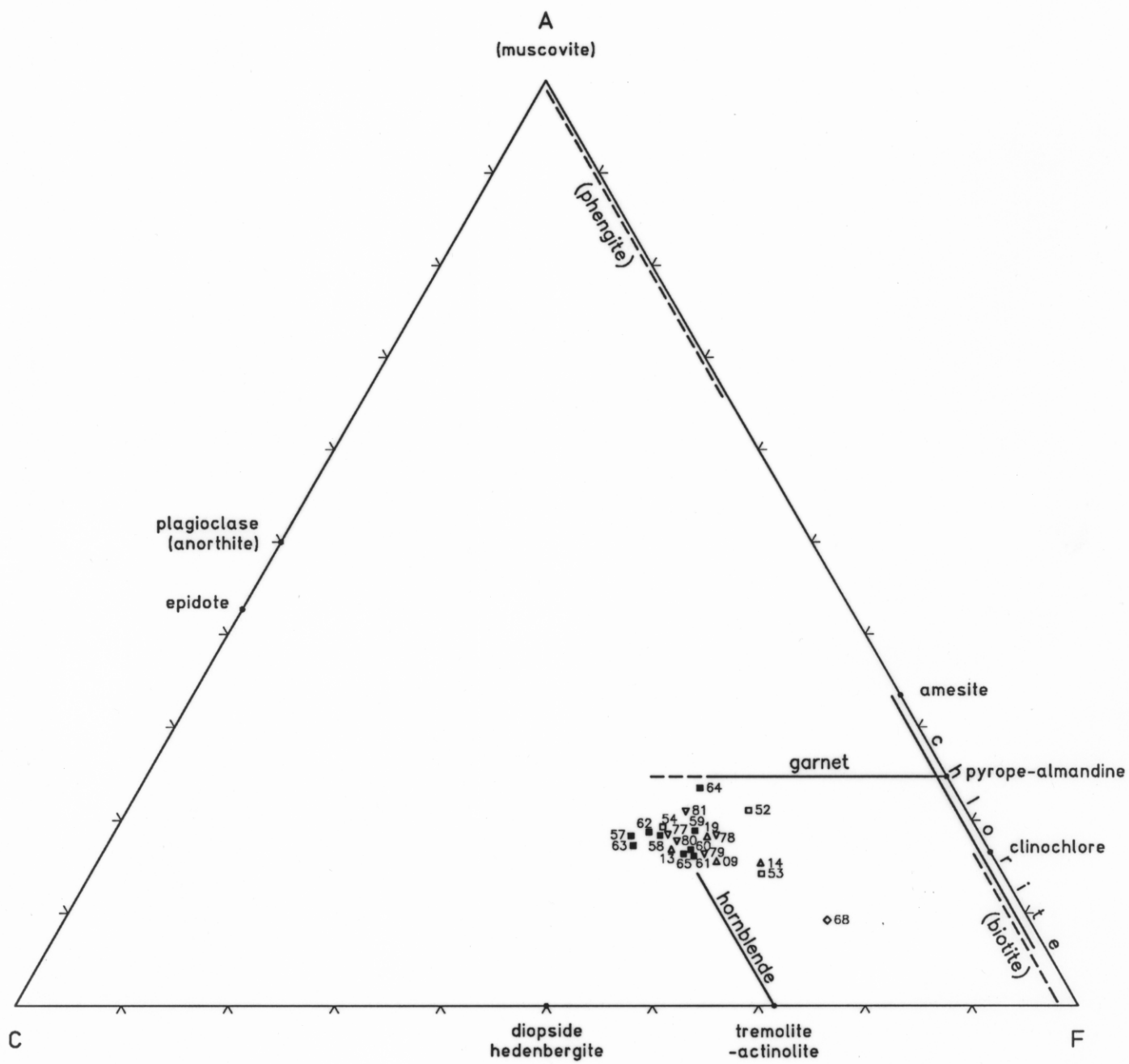
TYENNAN GEANTICLINE, METABASITES ON A-C-F DIAGRAM FIGURE No. U/R 1987/07 AUTHOR: J.L. EVERARD DIVISION OF MINES & MINERAL RESOURCES DRAFTSPERSON: ASM 27/02/90 5335F
