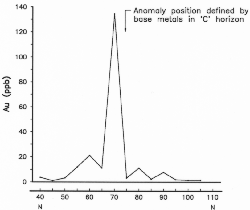
Fig. 5 Hument traverse profile (5810E) across Narrawa anomaly
