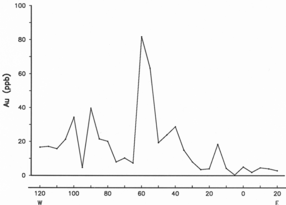
Fig.4 Hument traverse profile (65N) across Henty Fault zone north of Henty gold prospect
