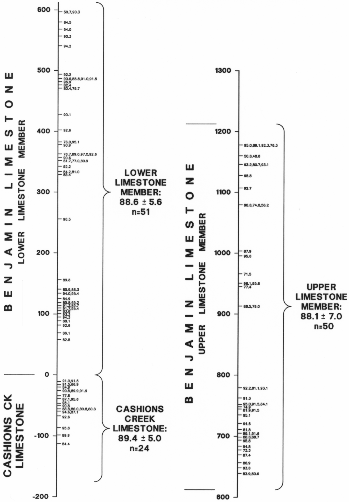
FLORENTINE VALLEY, CaCO 3 CONTENTS (%) OF SAMPLES FROM WESTFIELD SECTION FIGURE 8 REPORT 1990/06 AUTHOR: C.R. CALVER DIVISION OF MINES & MINERAL RESOURCES DRAFTSPERSON: ASM 26/03/90 5339H
