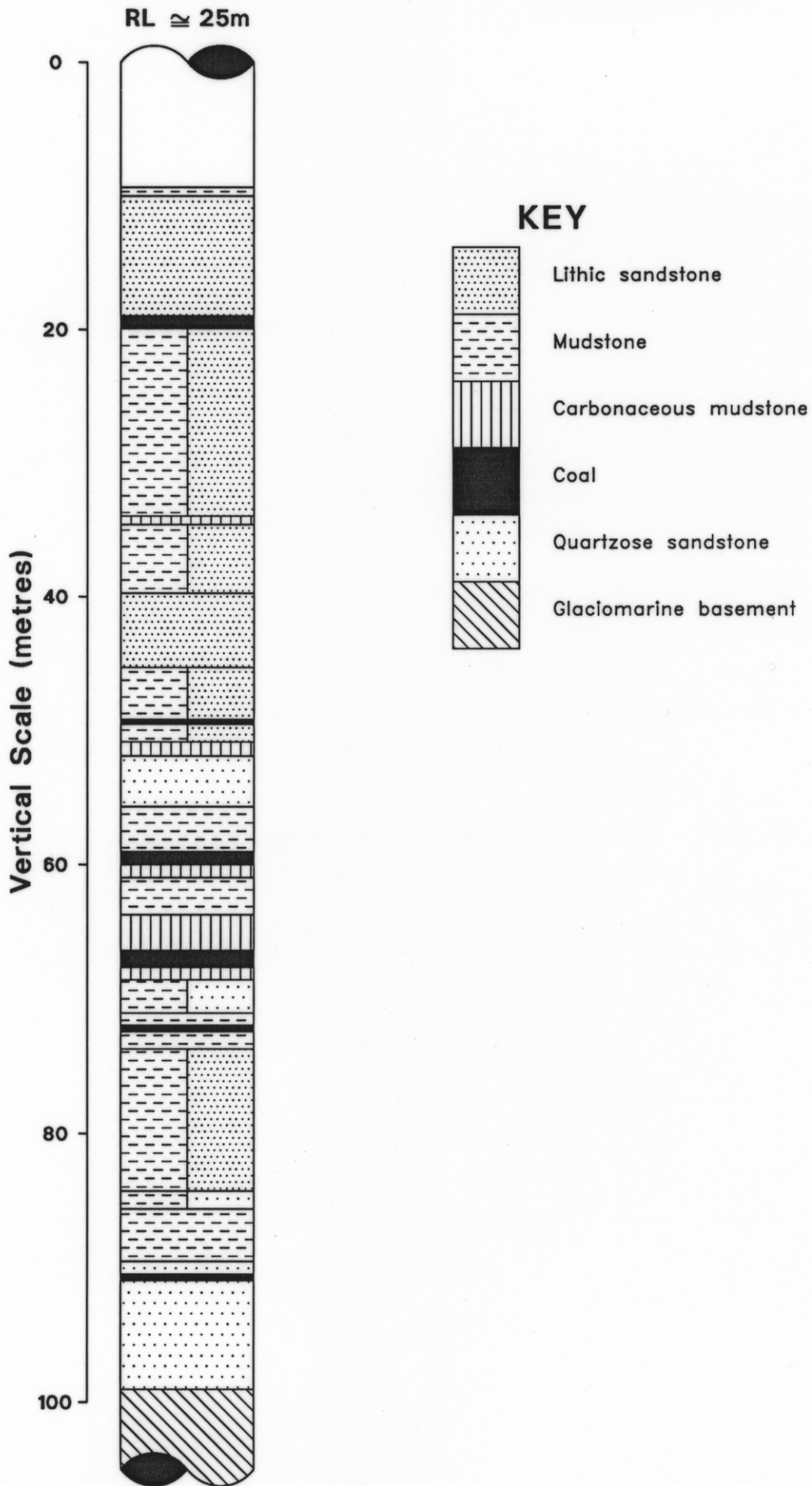
BICHENO, LOG OF DOM DDH 10 FIGURE No. COAL BULLETIN 64 AUTHOR: C.A. BACON DIVISION OF MINES & MINERAL RESOURCES DRAFTSPERSON: ASM 12/06/90 / 5343H
