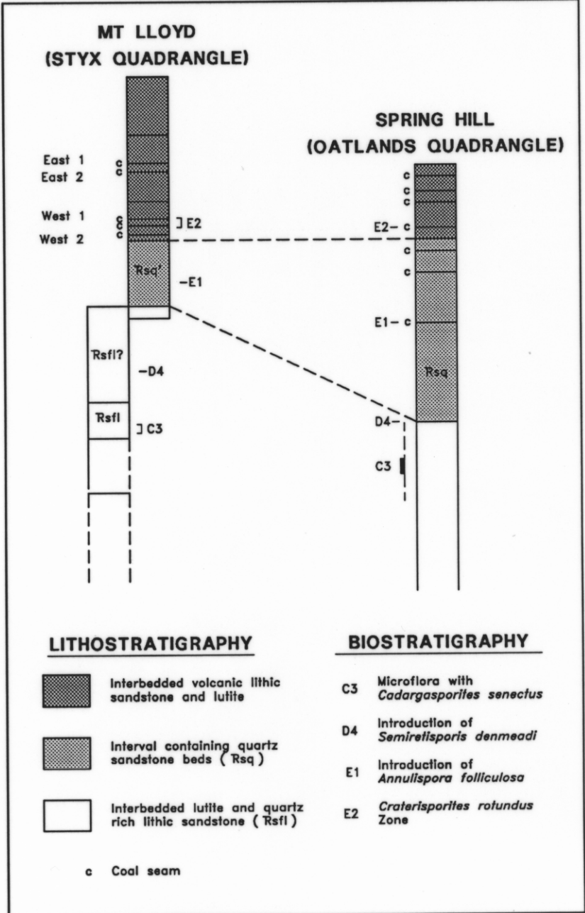
MT LLOYD & SPRING HILL, COMPARISON OF LITHOSTRATIGRAPHIC AND BIOSTRATIGRAPHIC RELATIONSHIPS FIGURE No. COAL BULLETIN AUTHOR: S.M. FORSYTH DIVISION OF MINES & MINERAL RESOURCES DRAFTSPERSON: ASM 03/07/90 5343M
