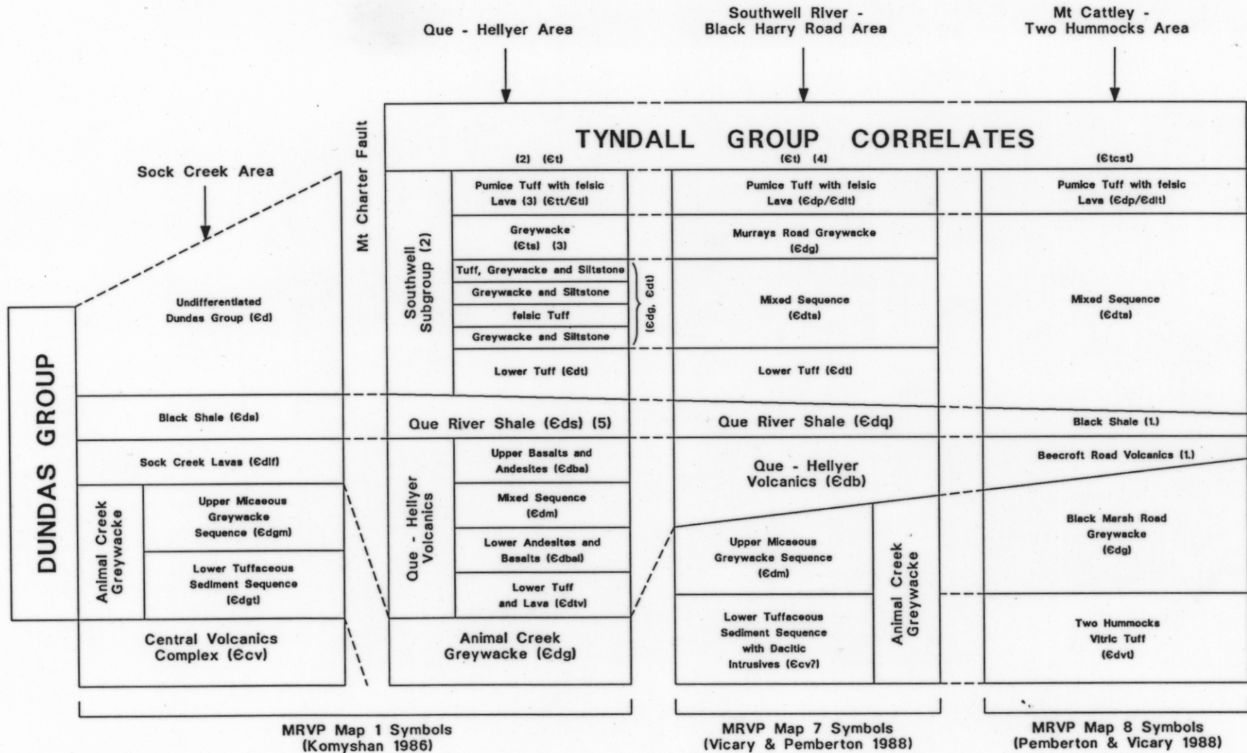
QUE-HELLYER - MT CATTLEY, SCHEMATIC STRATIGRAPHY FIGURE No. MRV REPORT 4 AUTHOR: M. VICARY DIVISION OF MINES & MINERAL RESOURCES DRAFTSPERSON: ASM 29/06/90 5349D
