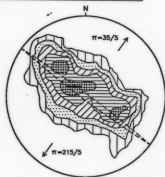
BACK PEAK - MT TOR AREA, (MAP 7&8) STRUCTURE STEREOPLOTS FIGURE XX TASMANIA DEPARTMENT OF MINES, MRV REPORT 4 AUTHOR: M. VICARY DRAFTSPERSON: ASM 25/06/80 5349E
