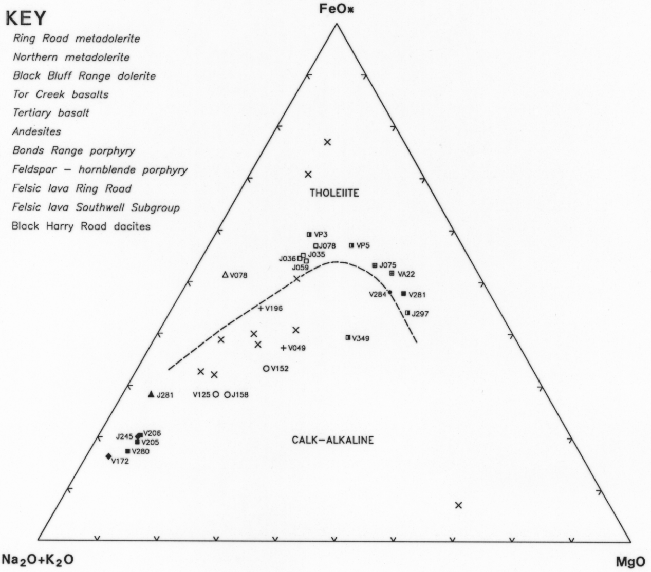
BACK PEAK - MT TOR AREA, (MAP 7&8) PLOT OF Na 2 O+K 2 O - MgO - FeO* FIGURE No. MRV REPORT 4 AUTHOR: M. VICARY DIVISION OF MINES & MINERAL RESOURCES DRAFTSPERSON: ASM 29/06/90 5349G
