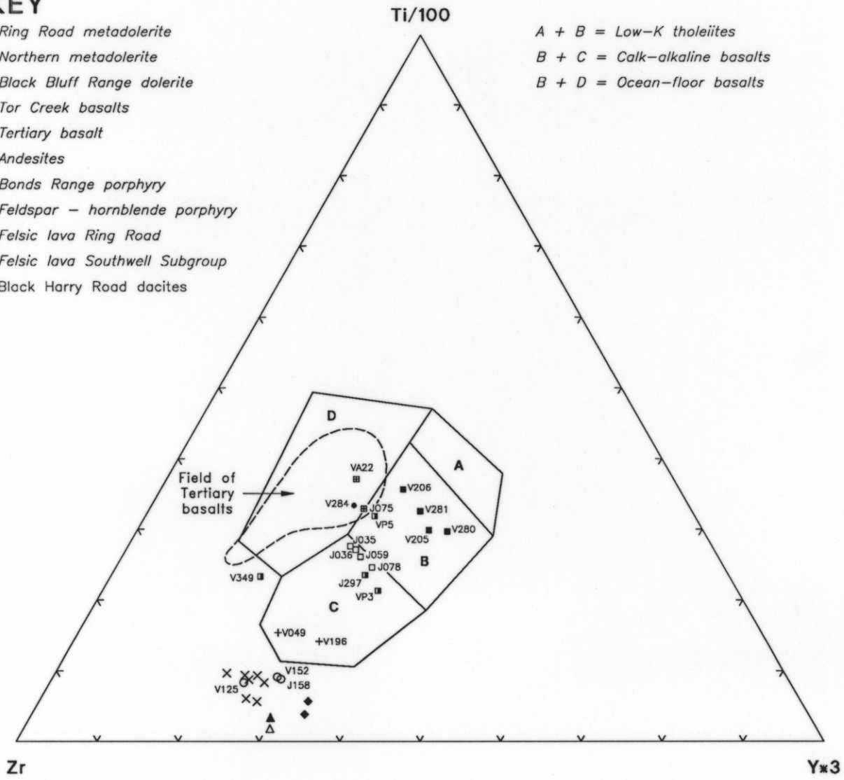
BACK PEAK - MT TOR AREA, (MAP 7&8) PLOT OF Zr - Ti/100 - Y*3 FIGURE No. MRV REPORT 4 AUTHOR: M. VICARY DIVISION OF MINES & MINERAL RESOURCES DRAFTSPERSON: ASM 29/06/90 5349H
