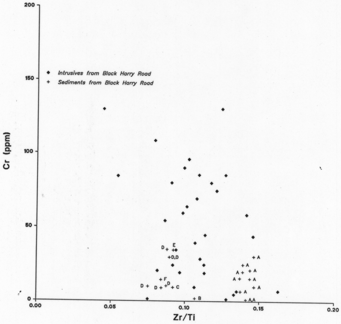
BLACK HARRY RD, (MAP 7&8) PLOT OF Zr/TI vs Cr FIGURE No. MRV REPORT 4 AUTHOR: M. VICARY DIVISION OF MINES & MINERAL RESOURCES DRAFTSPERSON: ASM 29/06/90 5349N
