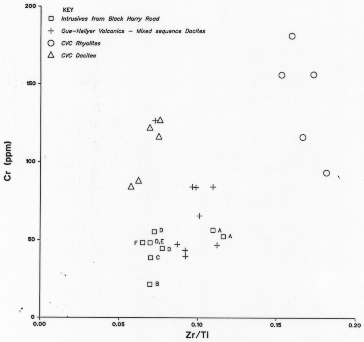
BLACK HARRY RD, (MAP 7&8) PLOT OF Zr/TI vs Cr FIGURE No. MRV REPORT 4 AUTHOR: M. VICARY DIVISION OF MINES & MINERAL RESOURCES DRAFTSPERSON: ASM 29/06/90 5349P
