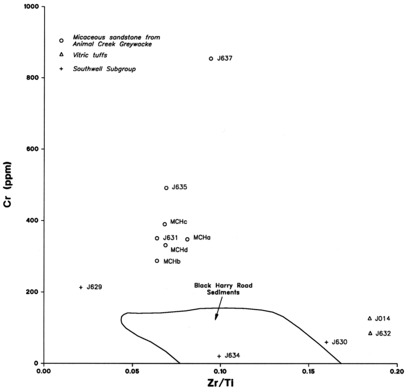
MT CATTLEY - HELLYER, (MAP 7&8) PLOT OF Zr/TI vs Cr FIGURE No. MRV REPORT 4 AUTHOR: M. VICARY DIVISION OF MINES & MINERAL RESOURCES DRAFTSPERSON: ASM 29/06/90 5349Q
