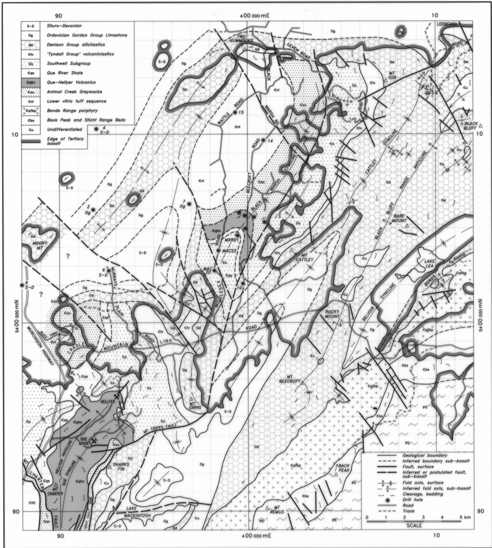
FIGURE 19. SUB-BASALT MAP AND STRUCTURAL MAP OF THE HELLYER - TWO HUMMOCKS - BLACK BLUFF RANGE AREA Pemberton et al. MRVP Geol. Rep.4 1991.
