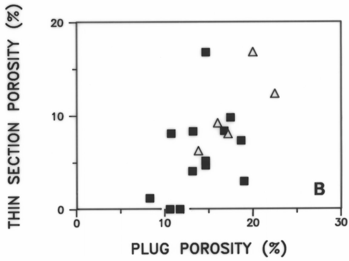
BASS BASIN, CORE PLUG AND PETROLOGICAL PLOTS, LOWER EASTERN VIEW GROUP FIGURE 13 APEA JOURNAL AUTHOR: P.W. BAILLIE DIVISION OF MINES & MINERAL RESOURCES DRAFTSPERSON: ASM 05/10/90 5358L
