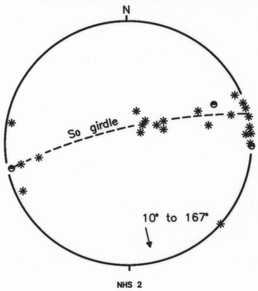
ST HELENS QUAD, STRUCTURAL STEREOPLOTS, NHS-2 TO NHS-7 FIGURE NHS2-7 ST HELENS EXPL NOTES AUTHOR: N.J. TURNER DIVISION OF MINES & MINERAL RESOURCES DRAFTSPERSON: ASM 21/2/92 5381A
