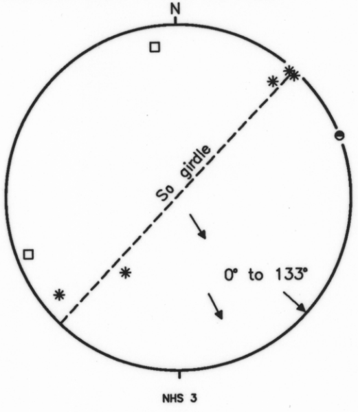
ST HELENS QUAD, STRUCTURAL STEREOPLOTS, NHS-2 TO NHS-7 FIGURE NHS2-7 ST HELENS EXPL NOTES AUTHOR: N.J. TURNER DIVISION OF MINES & MINERAL RESOURCES DRAFTSPERSON: ASM 21/2/92 5381A
