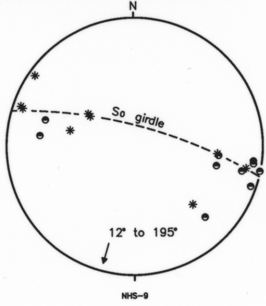
ST HELENS QUAD, STRUCTURAL STEREOPLOTS, NHS-8 TO NHS-13 FIGURE NHS8-13 ST HELENS EXPL. REPORT. AUTHOR: N.J. TURNER DIVISION OF MINES & MINERAL RESOURCES DRAFTSPERSON: ASM 21/1/92 5381B
