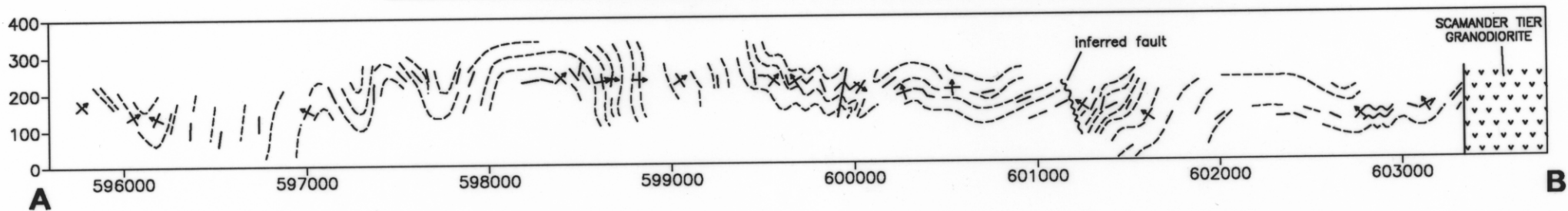
ST HELENS QUAD - MATHINNA BEDS, STRUCTURAL PROFILE (SECTN) ALONG GRID LINE 541500MN FIGURE 17 ST HELENS EXPL. REPORT. AUTHOR: M.P. McCLENAGHAN TASMANIA DIVISION OF MINES & MINERAL RESOURCES DRAFTSPERSON: ASM 21/2/92 5381 J
