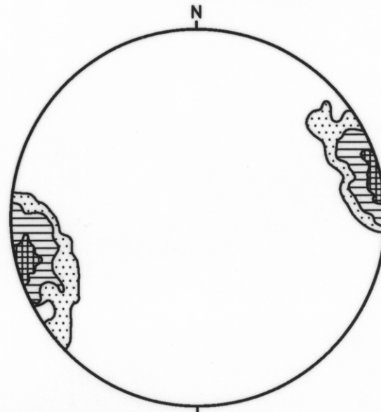
FIG 12. CONTOURED POLES TO CLEAVAGE, DOMAINS 3,4,5,6
