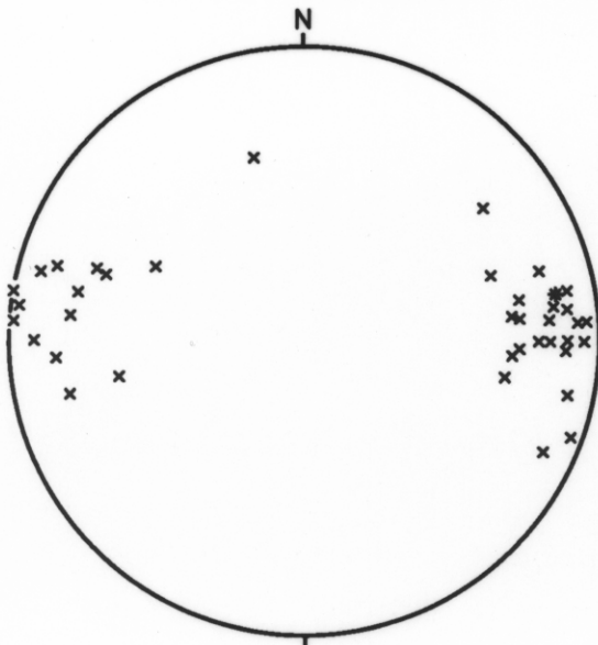
FIG 9, POLES TO BEDDING, DOMAIN 2
