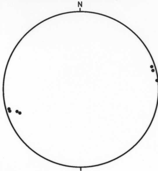
FIG 8, POLES TO CLEAVAGE, DOMAIN 1
