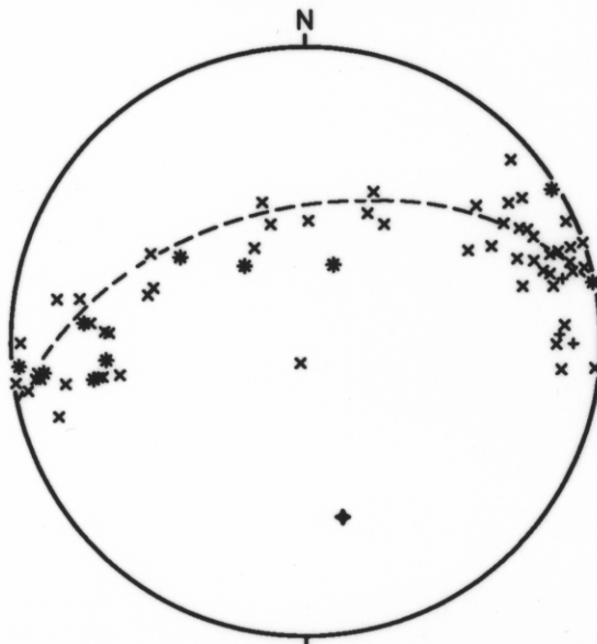
FIG 11. POLES TO BEDDING, DOMAINS 3,4,5,6
