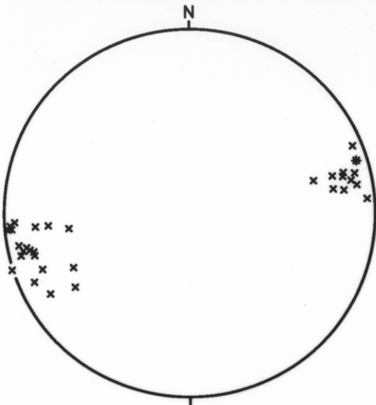
FIG 7, POLES TO BEDDING, DOMAIN 1
