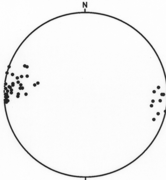
FIG 10, POLES TO CLEAVAGE, DOMAIN 2
