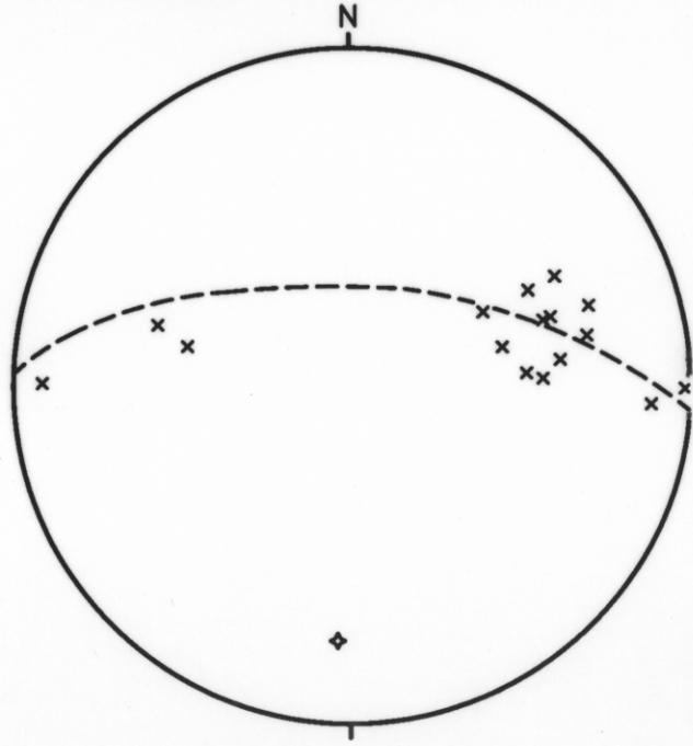
FIG 14, POLES TO BEDDING, DOMAIN 8
