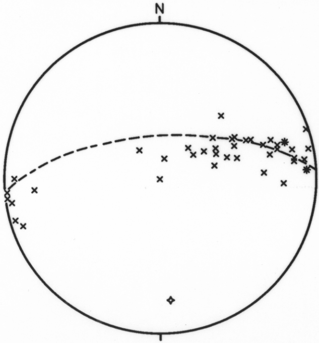
FIG 13, POLES TO BEDDING, DOMAIN 7
