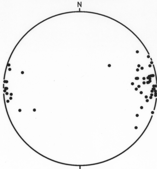
FIG 16, POLES TO CLEAVAGE, DOMANIN 9
