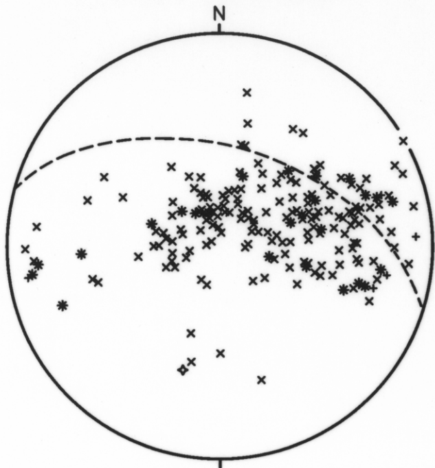
FIG15, POLES TO BEDDING, DOMAIN 9
