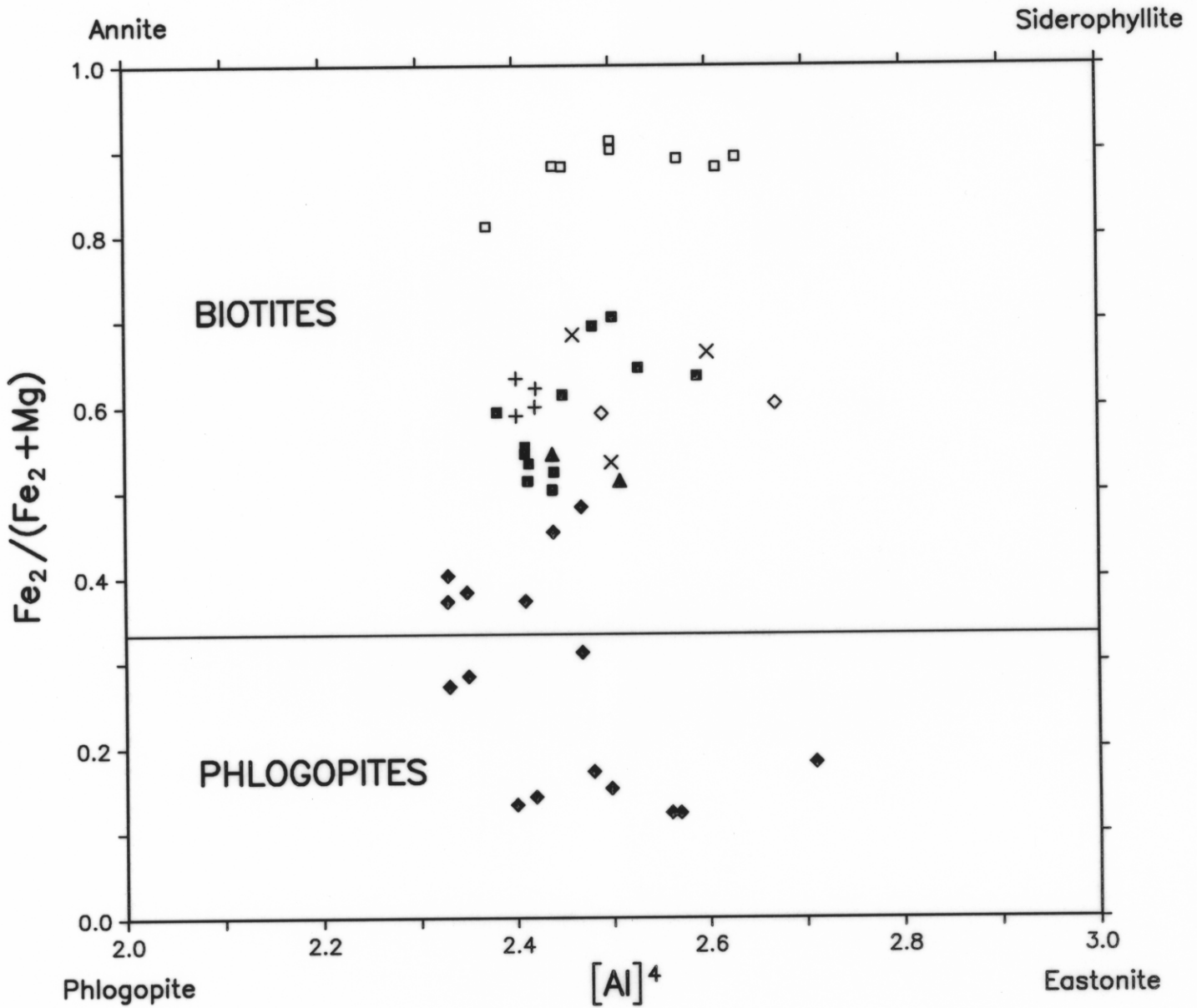
ST HELENS QUAD - MICA COMPOSITIONS (GRAPHS) FIGURE 3 ST HELENS EXPL. REPORT. AUTHOR: M.P. McCLEENAGHAN TASMANIA DEPARTMENT OF MINES DRAFTSPERSON: J. LADANIWSKYJ 26/3/92 5381 M
