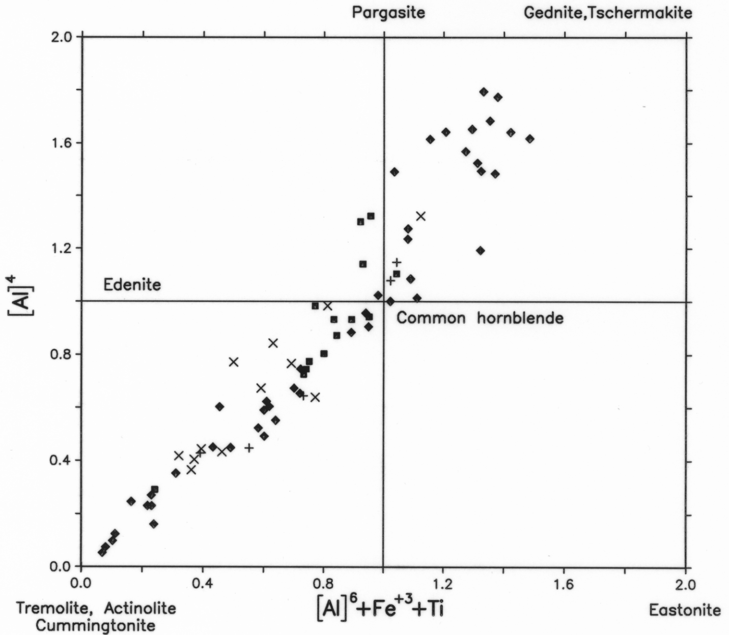
ST HELENS QUAD - AMPHIBOLE COMPOSITIONS (GRAPHS) FIGURE 4 ST HELENS EXPL. REPORT. AUTHOR: M.P. McCLENAGHAN TASMANIA DEPARTMENT OF MINES DRAFTSPERSON: J. LADANIWSKYJ 26/5/92 5381 N
