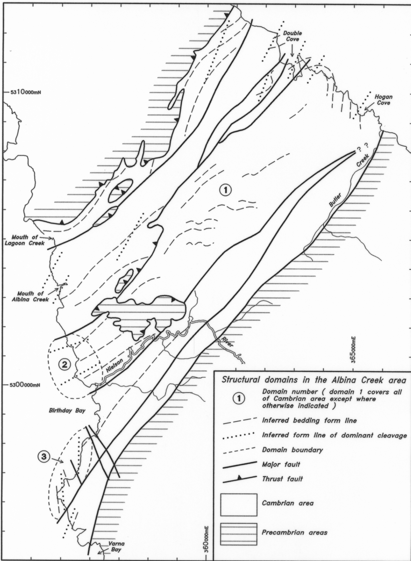
ALBINA CREEK, STRUCTURAL DOMAINS FIGURE 1a MACQUARIE HARBOUR EXPL. REPORT AUTHOR: M. MC CLENAGHAN DEPARTMENT OF MINES DRAFTSPERSON: ASM 11/03/92 5406A
