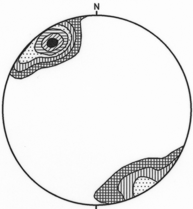
Fig.4a ALBINA CK AREA, DOMAIN 2, POLES TO DOMINANT S3 CLEAVAGE
