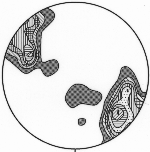
Fig.5n DOMAIN 1 – POLES TO BEDDING
