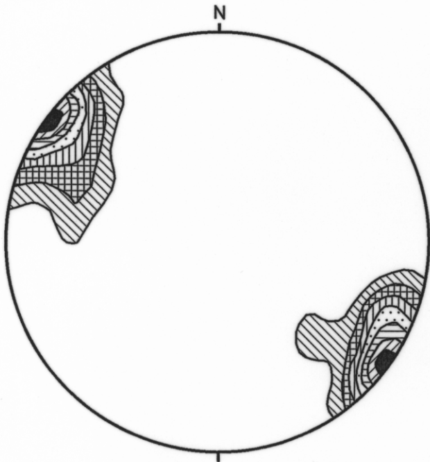
Fig.3n DOMAIN 1 – POLES TO S4
