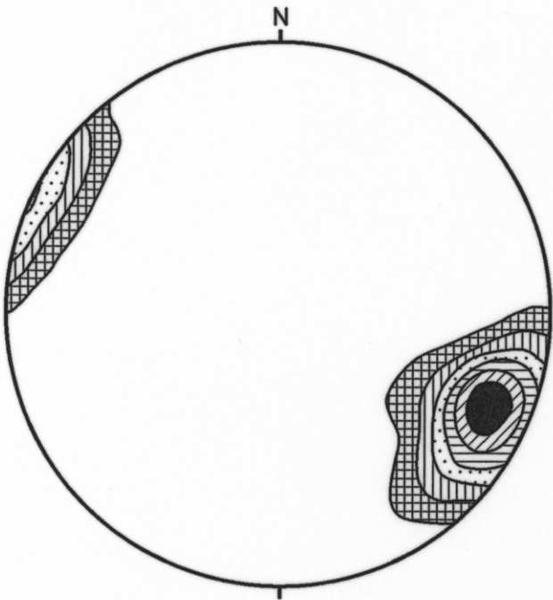
Fig.3c ALBINA CK AREA, DOMAIN 1, POLES TO DOMINANT S3 CLEAVAGE
