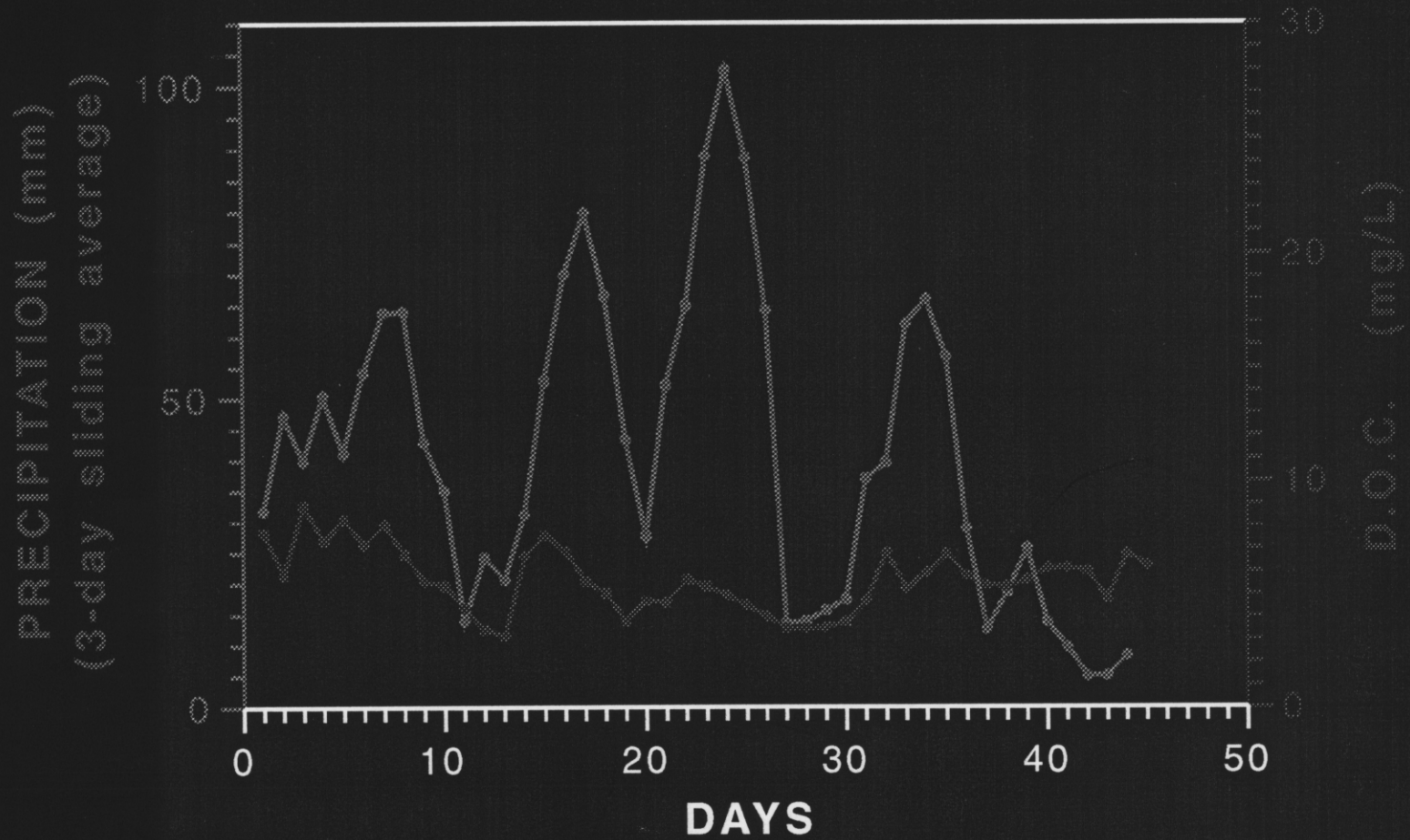
CONCENTRATION OF D.O.C. IN STERLING RIVER COMPARED TO PRECIPITATION. (Koehnken 1992)
