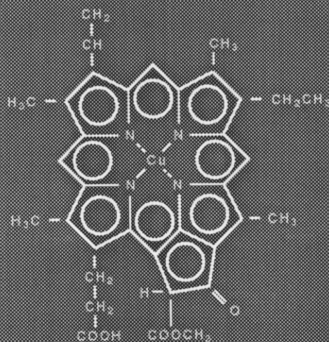
COPPER PORPHYRIN
