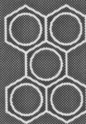
PERYLENE
