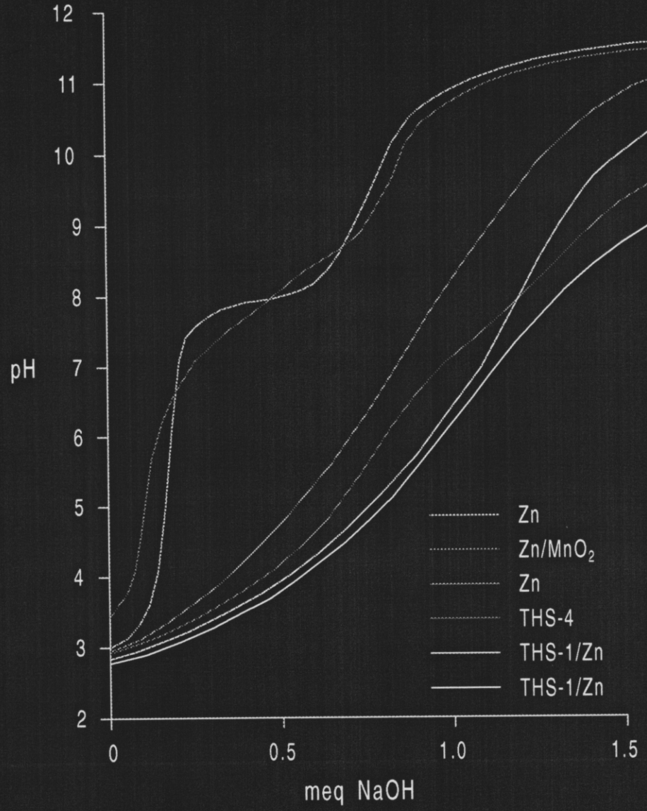
POTENTIOMETRIC TITRATION CURVES FOR 500meq ZINC ALONE AND IN THE PRESENCE OF 0.2g MnO 2 , THS-1 AND THS-4
