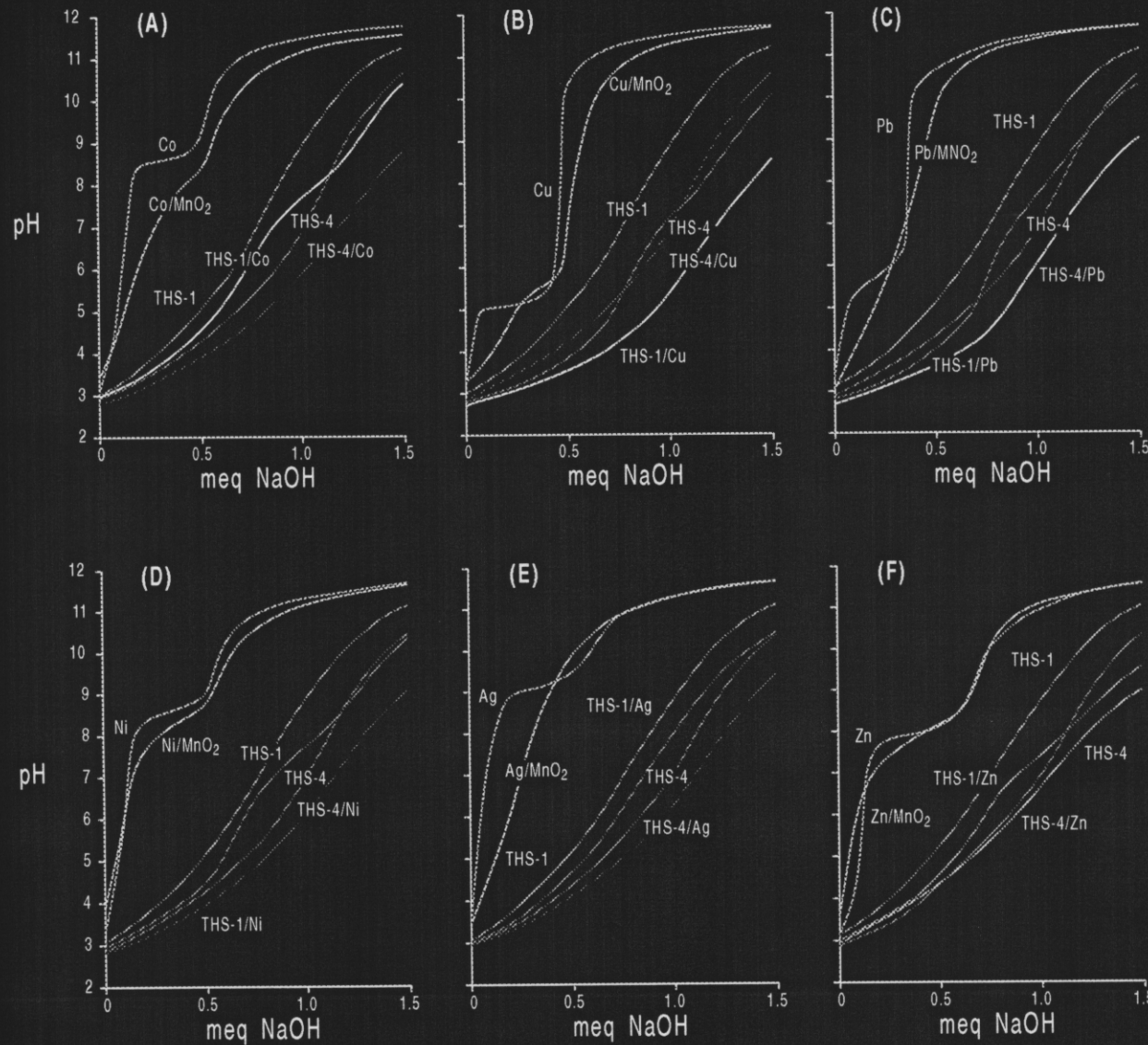
POTENTIOMETRIC TITRATION CURVES FOR 500 meq OF: (A) COBALT, (B) COPPER, (C) LEAD, (D) NICKEL, (E) SILVER) AND (F) ZINC, ALONE AND IN PRESENCE OF 0.2g MnO 2 , THS-1 AND THS-4
