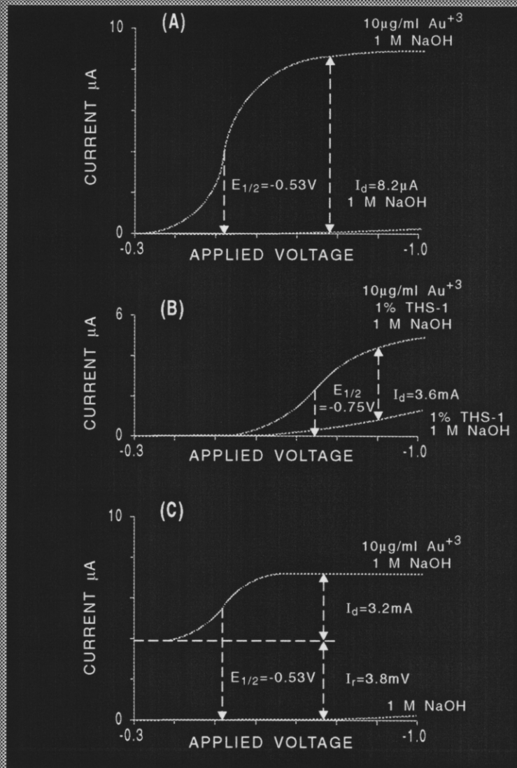
POLAROGRAMS OF : (A) 10 μg/ml Au 3+ in 1 M NaOH (B) as for (A) with addition of THS-1 (C) repeat of (A) after lapse of 24 hours.
