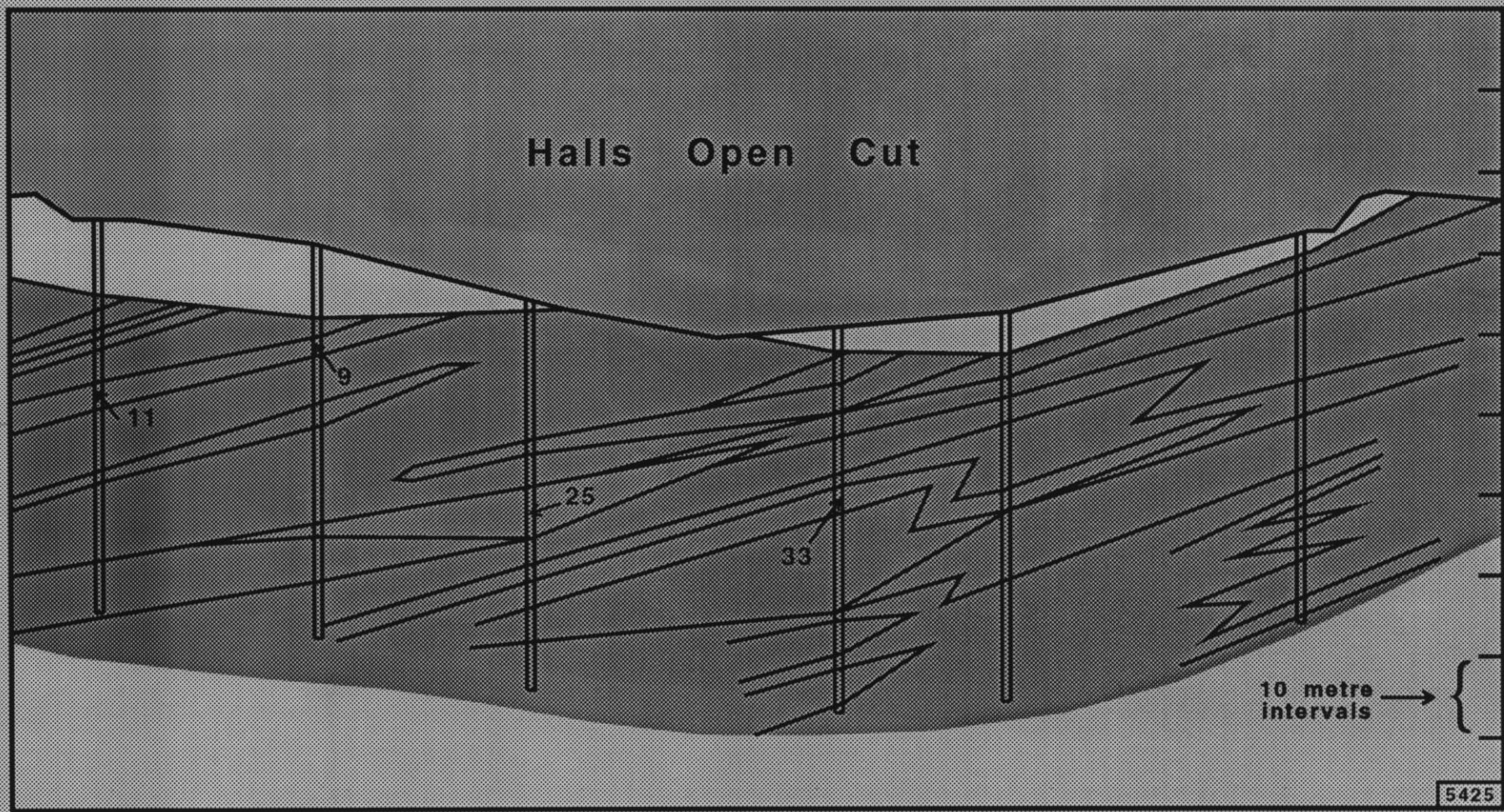
Schematic diagram of Halls Open Cut - Adamsfield
