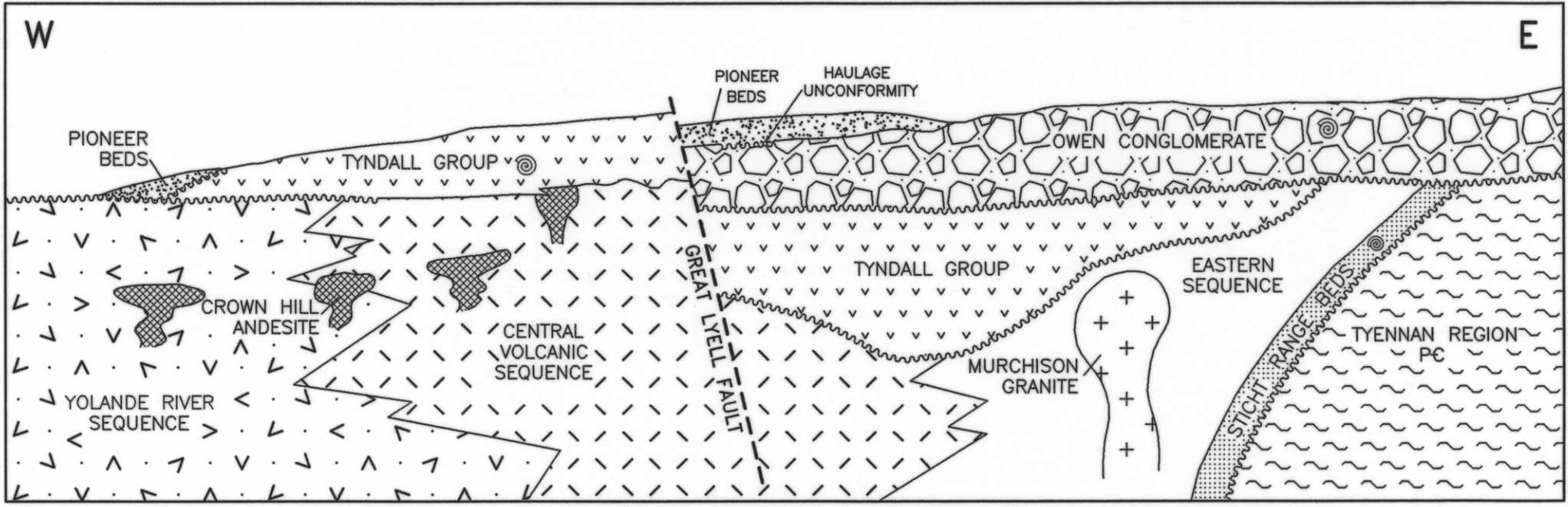
SCHEMATIC CROSS-SECTION, MT. READ VOLCANICS, QUEENSTOWN AREA
