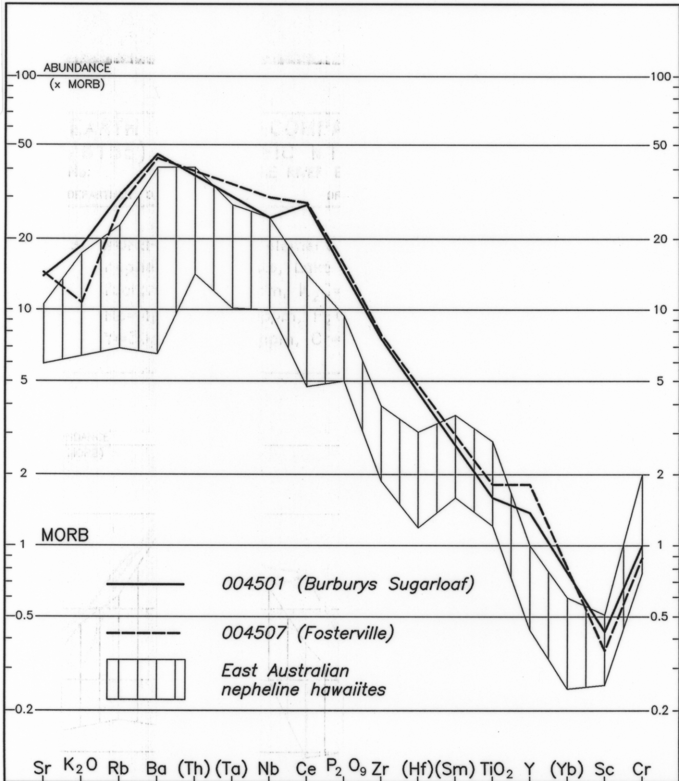
Figure B MORB-normalised element abundancies for nepheline hawaiiite and nepheline mugearite, Lake River quadrangle. MORB normalisation factors (Sr=120ppm, K 2 O=0.15%, Rb=2ppm, Ba=20ppm, Nb=4ppm, Ce=10ppm, P 2 O 9 =0.12%, Zr=90ppm, TiO 2 =1.5%, Y=30ppm, Sc=40ppm, Cr=250ppm) from Pearce.(1980)
