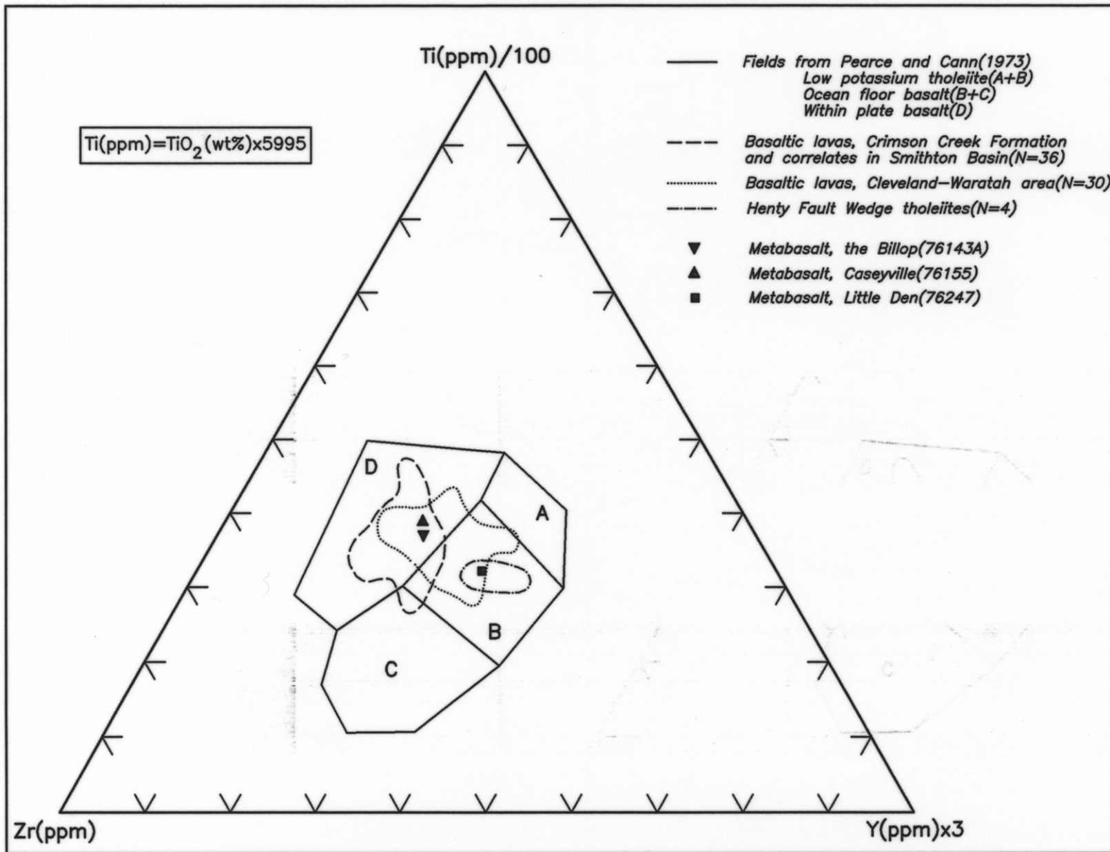
Ti-Zr-Y DIAGRAM ?PROTEROZOIC / ?CAMBRIAN METABASALTS FIGURE No. REPORT: LAKE RIVER EXPLANATORY NOTES AUTHOR: J.L.EVERARD MINERAL RESOURCES TASMANIA DRAFTSPERSON: A.J.HOLLICK 15/11/93 5441P
