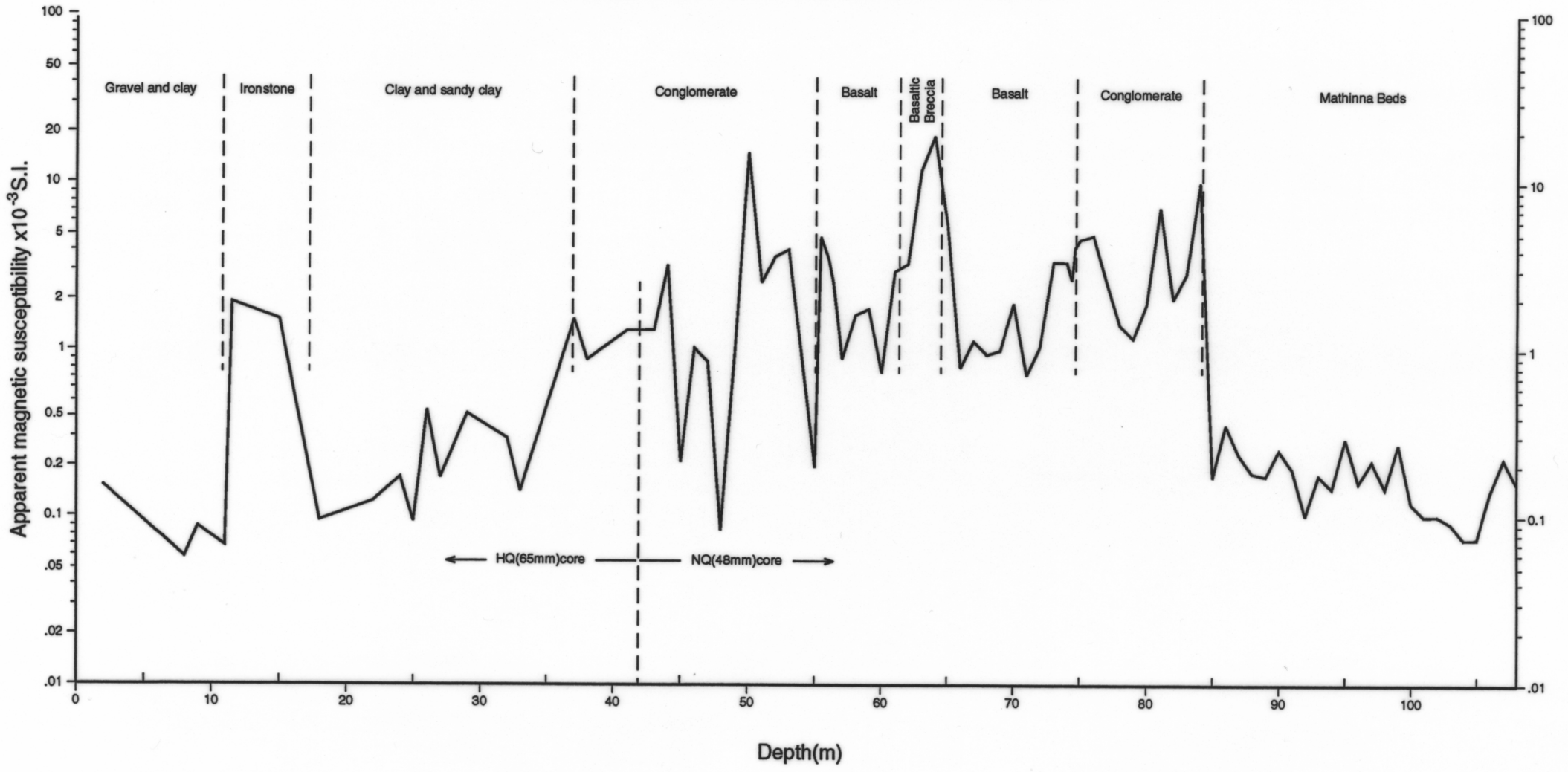
MALAHIDE INSIDE PLAIN DDH APPARENT MAGNETIC SUSCEPTIBILITY OF CORE FIGURE No. REPORT: AUTHOR: J.L.EVERARD MINERAL RESOURCES TASMANIA DRAFTSPERSON: A.J.HOLLICK 10/1/99 5460A
