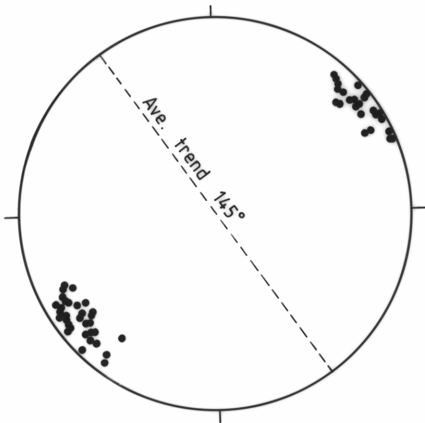
NW-SE trending cleavage (poles)
