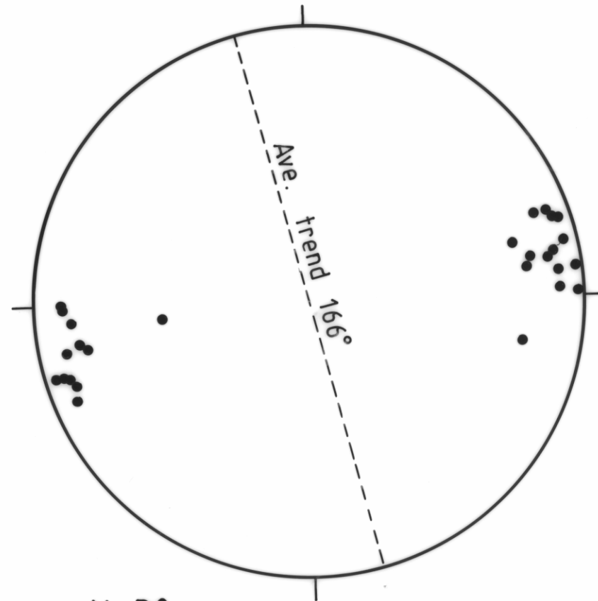
Other cleavages (poles)
