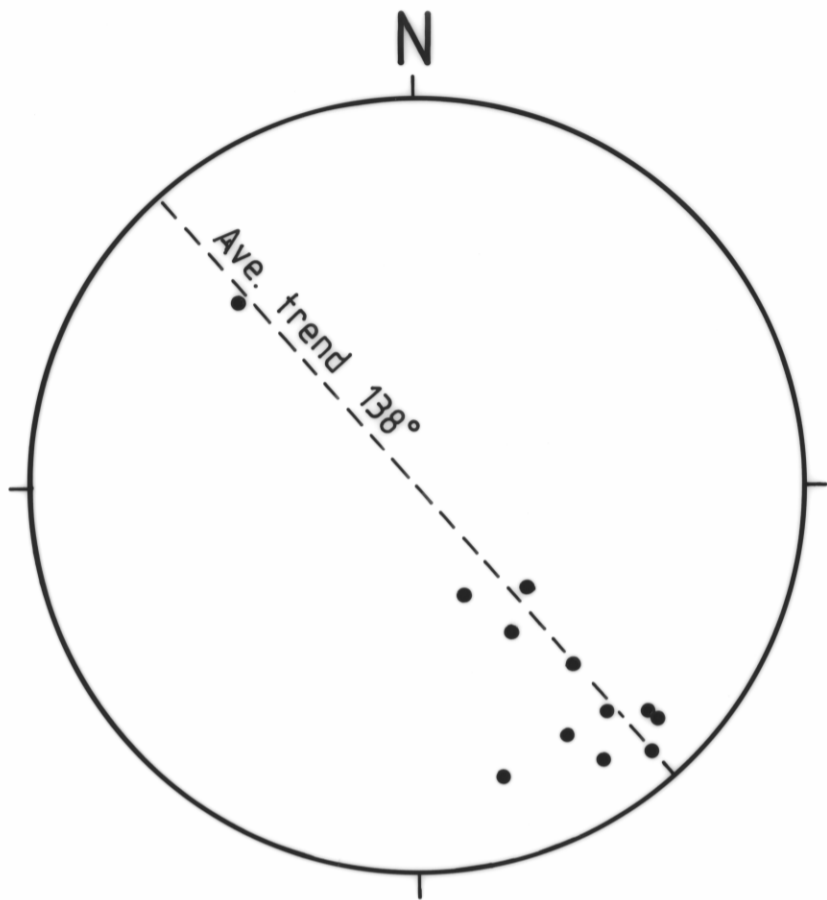
F 3 fold axes
