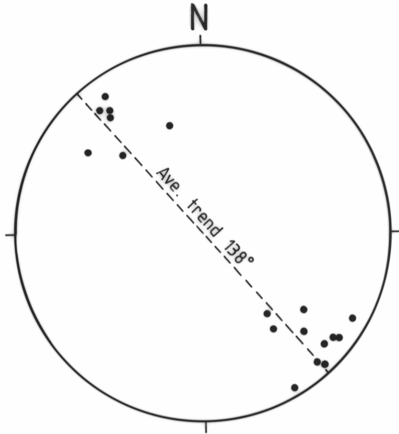
L 3 crenulation lineations
