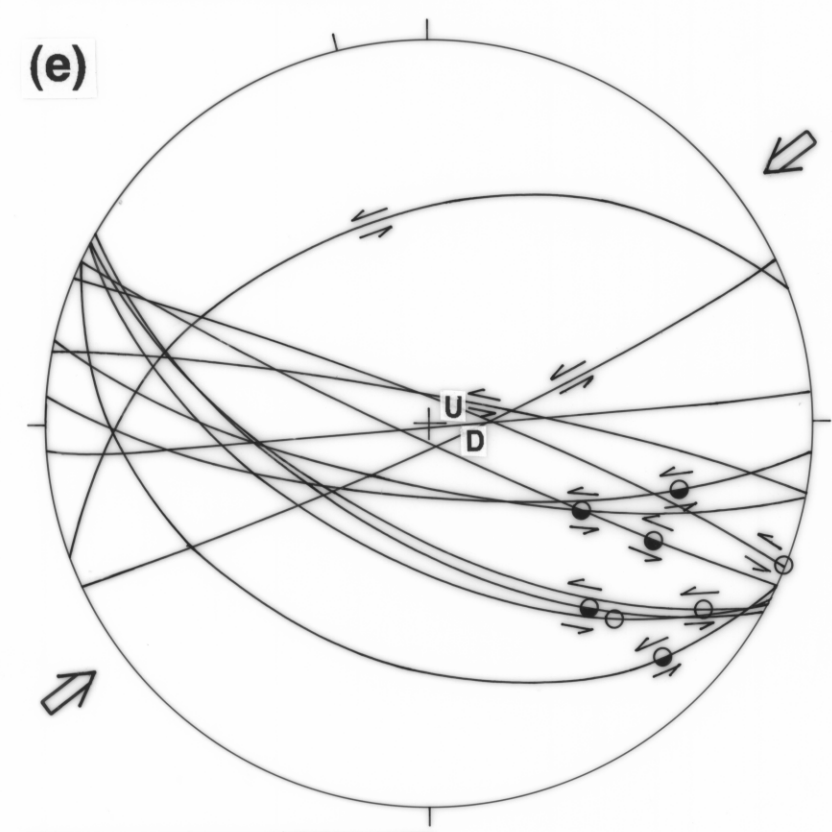
D 3 SINISTRAL WRENCH
