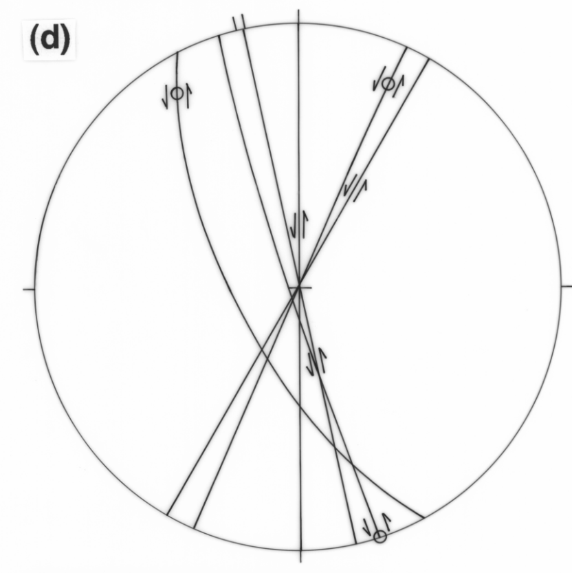
D 2 or D 3 SINISTRAL WRENCH
