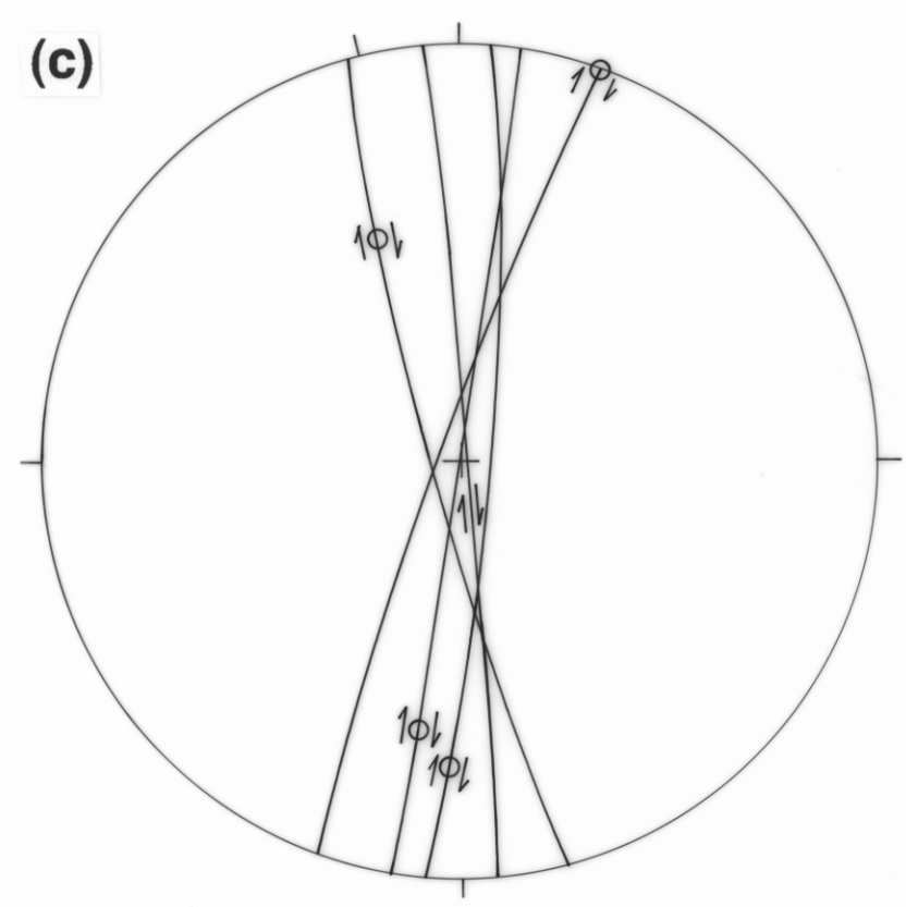
D 2 - DEXTRAL WRENCH
