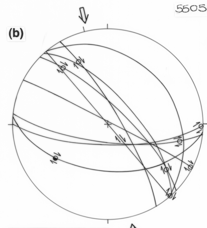
D 2 - DEXTRAL WRENCH
