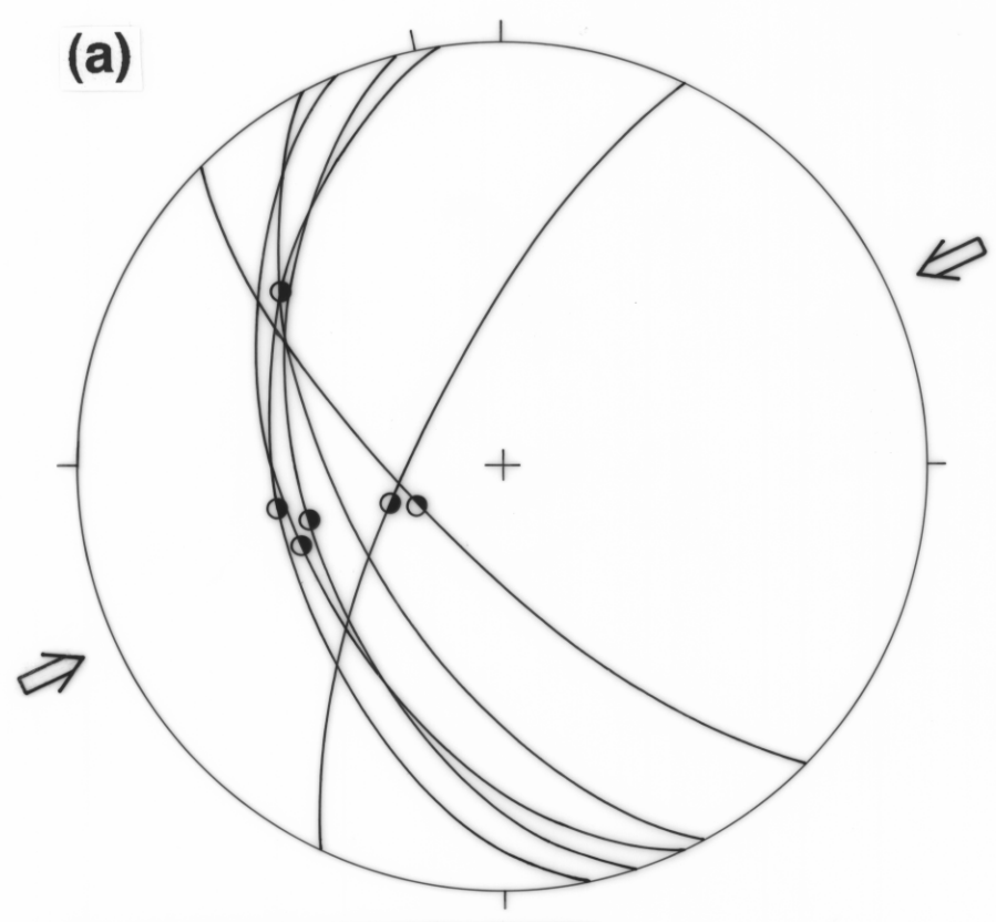
D 1 THRUSTS (NE-DIRECTED)
