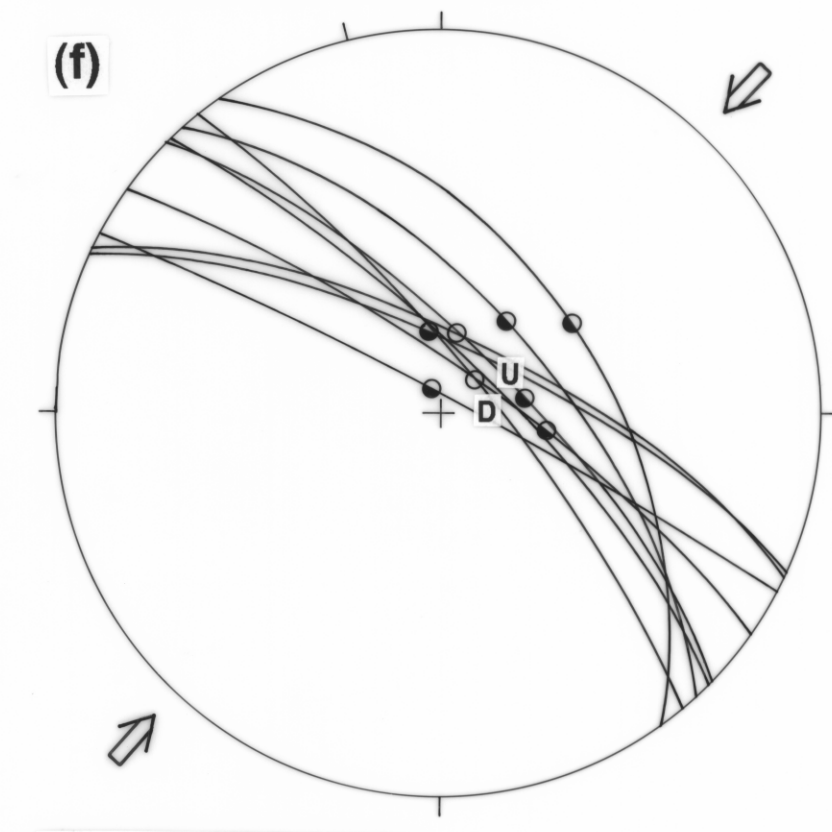
D 3 REVERSE FAULTS
