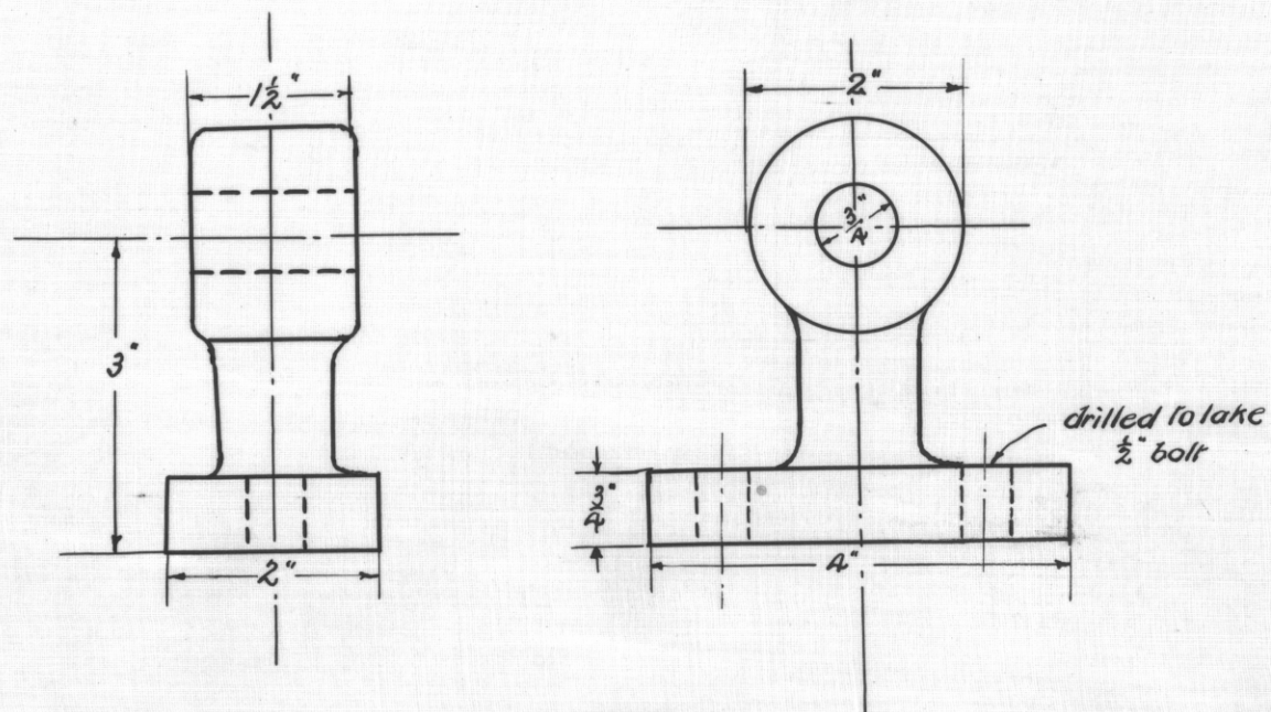
Details of Bearings \frac{1}{2} full size
