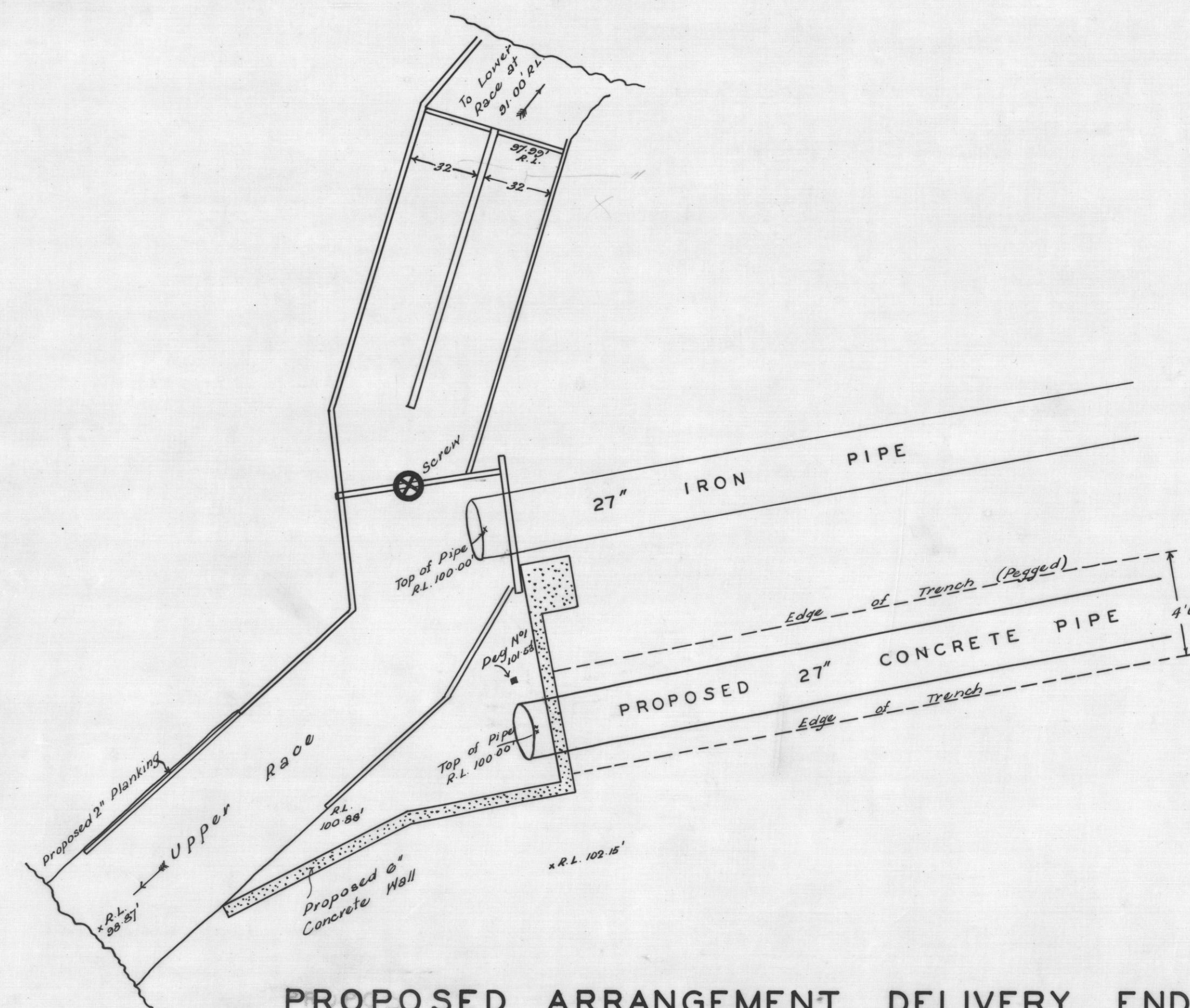
PROPOSED ARRANGEMENT DELIVERY END 1 INCH = 4 FEET
