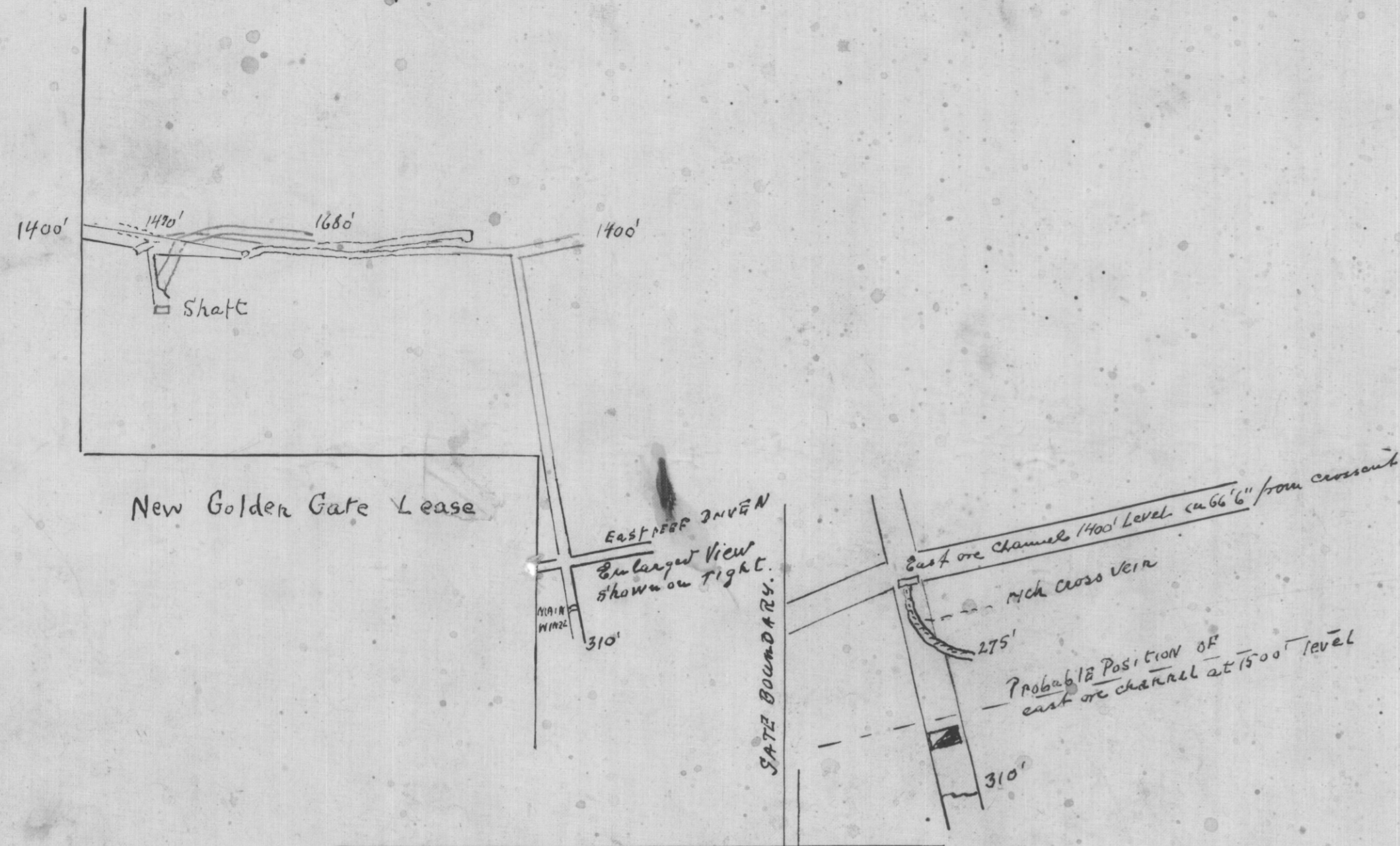
Plan of 1400', 1500', and 1600' Levels
