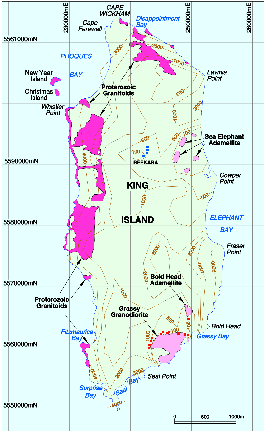
Fig 12. Interpreted granitoid depth contours with depth to top of granitoid shown in metres. Derived from MRT gravity data base by Leaman (2003). The pattern is thought to reflect extensive subsurface Devonian - Carboniferous granitoid (light pink) with little influence from Proterozoic granitoids (pink). Granitoid outcrops are from MRT 1 : 250,000 'Geology of Northwest Tasmania', Calver et al, 1995. W (■) and Sn/W (■) occurrences are from MRT Mirloch database. Grid is AMG, AGD66, Zone 55.
