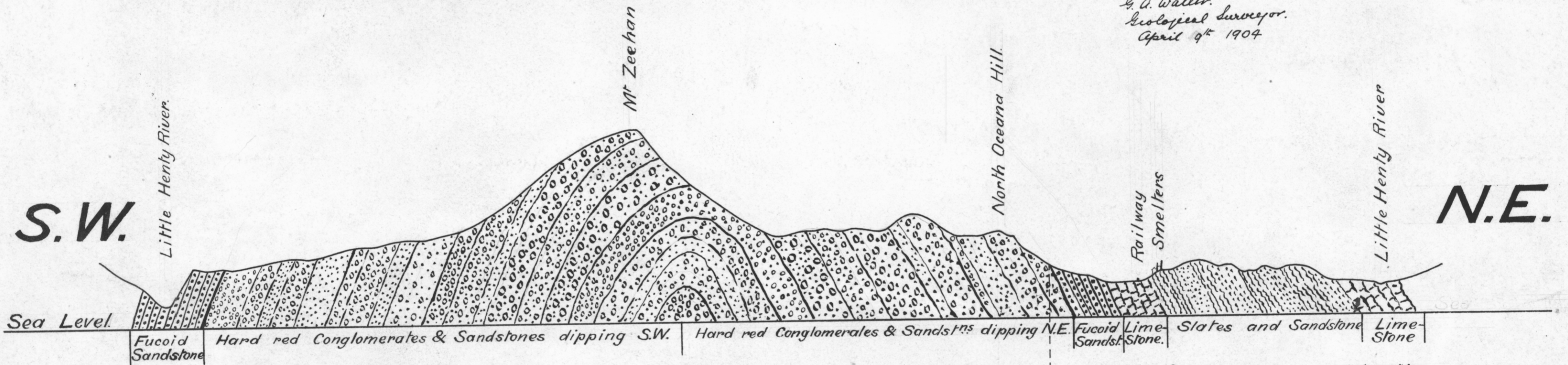
Fig 1. Ideal Section through Mt Zeehan on approximate bearing of 45° East of North
