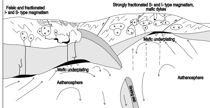
18c. Slab break-off and asthenospheric upwelling (~380 - 360Ma)
